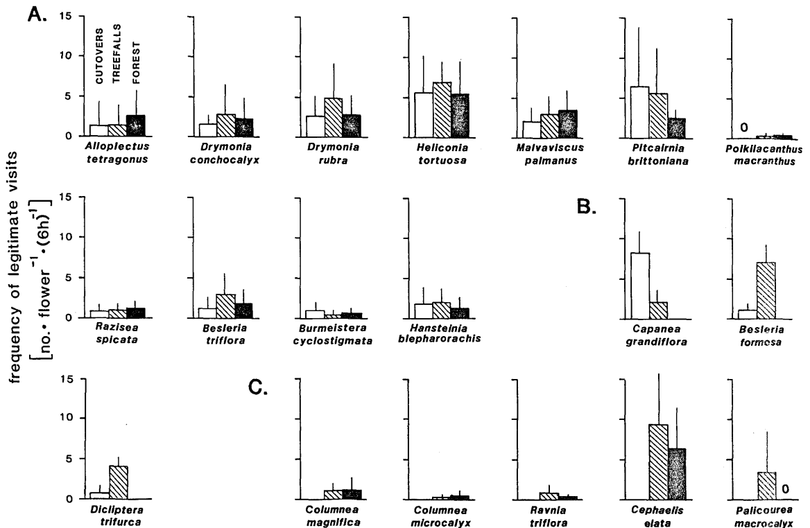
FIG. 1. Frequencies of legitimate (potentially pollinating) visits by hummingbirds to species observed at least three times (A) in each patch type; (B) in cutovers and treefalls only; (C) in treefalls and forest only. Height of bar indicates mean visit frequency over the \geq 3 observations, height of line above bar indicates standard deviation. In each subset (A, B, C), long-flowered species are listed first.
