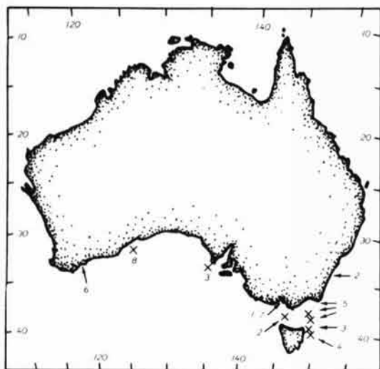
FIG. 3. Locations from which Xestoleberis has been reported from Australia: 1, Brady (1866); 2, Brady (1880); 3, Chapman (1915); 4, Chapman (1919); 5, Chapman (1941); 6, McKenzie (1964); 7, McKenzie (1967); 8, Chapman and Parr (1935).
