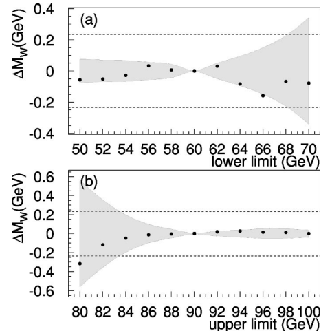
FIG. 18. Variation of the fitted W boson mass with (a) the lower edge and (b) the upper edge of the fit window for the transverse mass distribution. The shaded regions and the dashed lines are described in the text.
