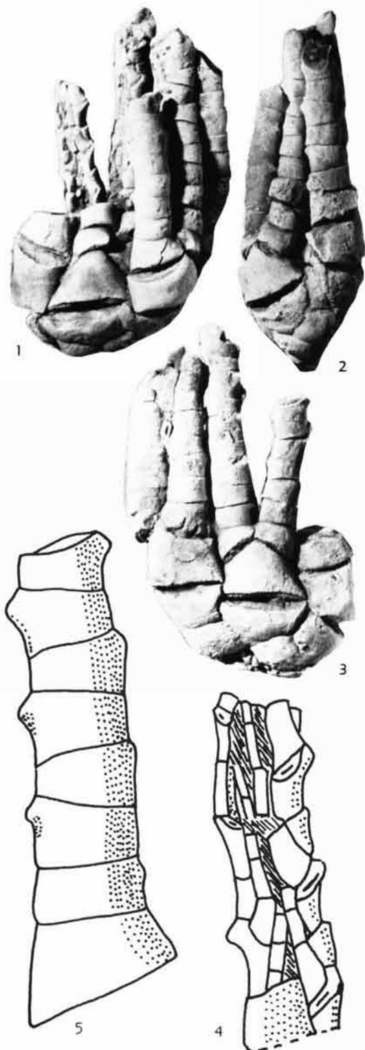
FIG. 3. Atrapocrinus mutatus Strimple, n. sp., from
