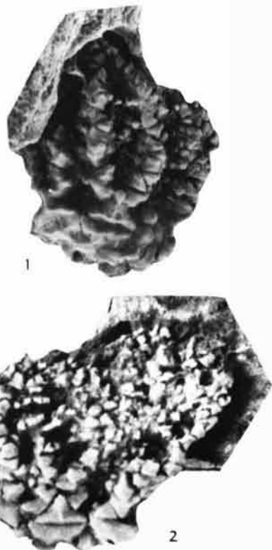
FIG. 7. Brabeocrinus primus Strimple, n. sp.—1, 2. Holotype crown (OU 7131) from Coal County, Oklahoma, viewed from D ray (posterior interray to right), and B ray, \times 2.8 .
