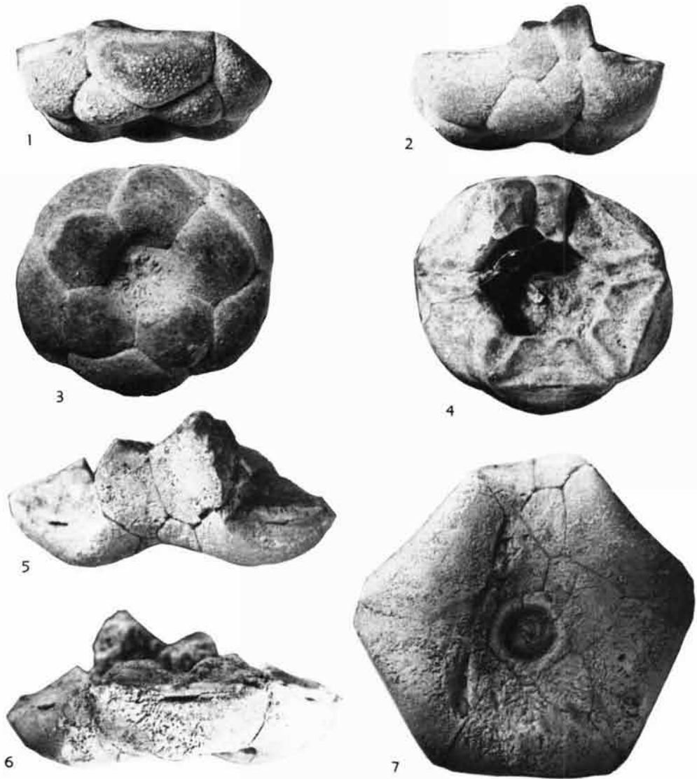
FIG. 12. Affinocrinus (1-4) and Sciadiocrinus (5-7) from Oklahoma and Missouri.—1-4. A. orbis , n. sp. Holotype cup, OU 7145, viewed from anterior, posterior, base, and summit, \times 4 .—5-7. S. plantus , n. sp. Holotype cup, USNM 144994, viewed from posterior, anterior, and base, \times 2.5 .
