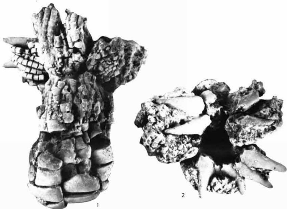
FIG. 14. Sciadiocrinus planulatus (Moore & Plummer) from Atoka Formation, Coal County, Oklahoma.—1, 2. Hypostome crown, OU 4478 side view and summit view showing spinose termination of anal sac, \times 3.0 .
