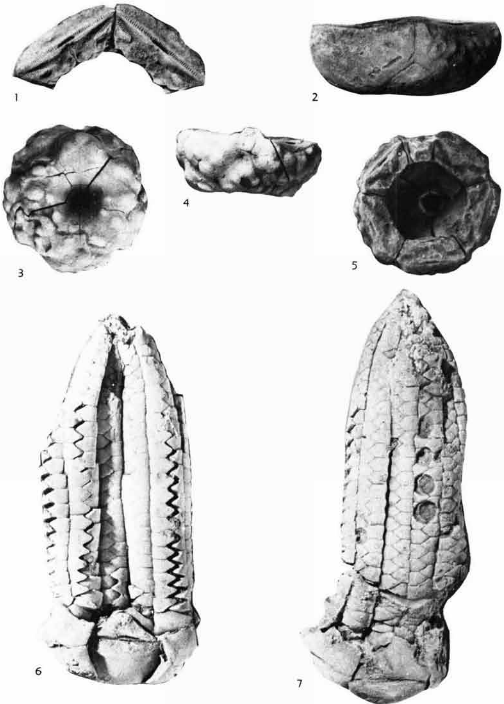
FIG. 10. Diphucrinus (1, 2) and Protencrinus (6, 7) from the Atoka Formation, and Graffhamicrinus (3-5) from the Bostwick Formation, Oklahoma. (Continued on facing page.)
