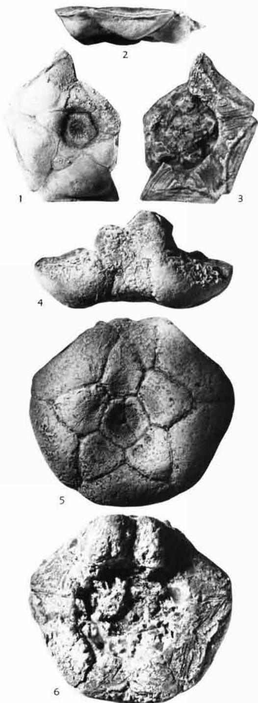
FIG. 13. Platyfundocrinus from Oklahoma and Missouri. —1-3. P. webbersensis , n. sp. Holotype cup, SUI 35597, from Atoka Fm., Wagoner Co., Okla.; viewed from base,
