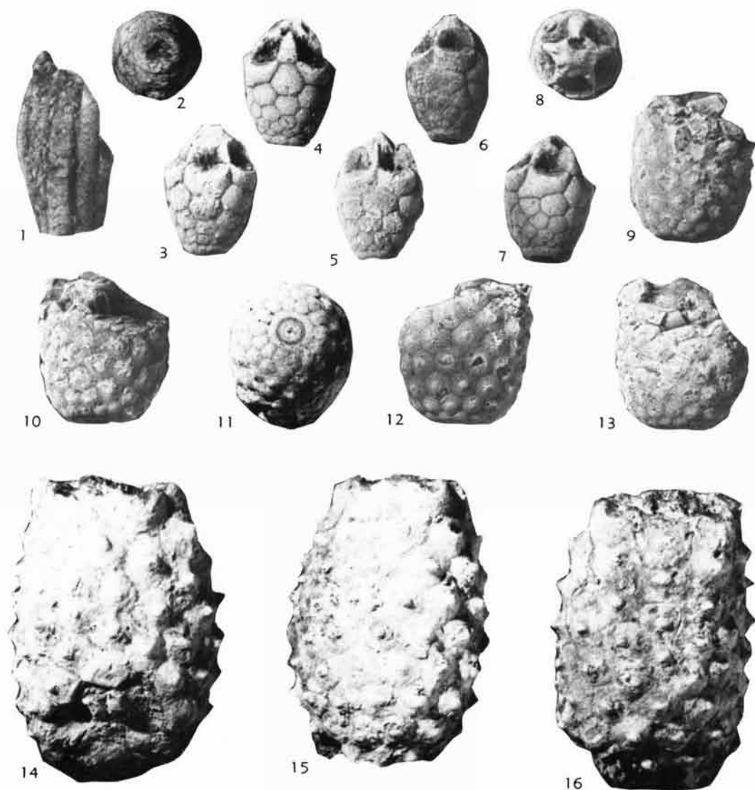
FIG. 17. Planacrocrinus (1-8) and Globoacrinus (9-16) from the Burgner Formation of Missouri.—1-8. P. knappi Strimple, n. sp.; 1, paratype (UM 14825b) arms; 2-8, holotype theca (UM 14825), base, anterior, posterior, AB interray, AE interray, C ray, summit, \times 3 .—9-16. G. centronodus Strimple, n. sp.; 9-13, paratype cup (USNM 144999a) from A ray, E ray, base, B ray, D ray; 14-16, holotype cup (USNM 144999) from AE interray, BE interray, CD interray, \times 3 .
