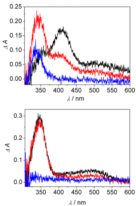
Figure 1. Transient absorption spectra of 7b in an water/acetonitrile (30:70, v/v) mixture without (top) and with (bottom) a drop of perchloric acid recorded 30 ns (black), 100 ns (red), and 5 \mu s (blue) after a 266 nm laser flash.
