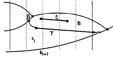
Figure 5: Proof of Lemma 9.
