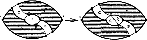
Figure 4: Inserting e = (\alpha, \beta) when \beta \prec_{\Pi} f \prec_{\Pi} \alpha ( A\beta B f C \alpha D \rightarrow A f_1 C \alpha e \beta B f_2 D ). A, B, C , and D are defined by the topmost path from s to \alpha and from s to \beta , and bottommost path from \alpha to t and from \beta to t .
