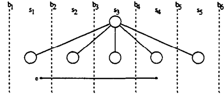
Figure 2: A node in the base tree. For segment e we have l = 1 , r = 4 . Its middle subsegment spans s_2 and s_3 .
