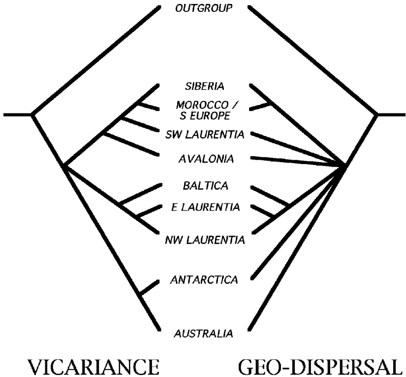
Figure 3 Paleobiogeographic patterns in Cambrian trilobites based on Lieberman (2003b,c), derived using the modified version of BPA described in the text. The most parsimonious pattern of vicariance and the strict consensus of the most parsimonious patterns of geo-dispersal are labeled. Laurentia refers to North America and Greenland, which were once conjoined; Baltica was a separate continent in the Cambrian, comprising Scandinavia and the eastern European platform; Avalonia refers to what was, in the Cambrian, a series of closely associated microcontinents including principally the eastern part of Newfoundland and much of Great Britain.
