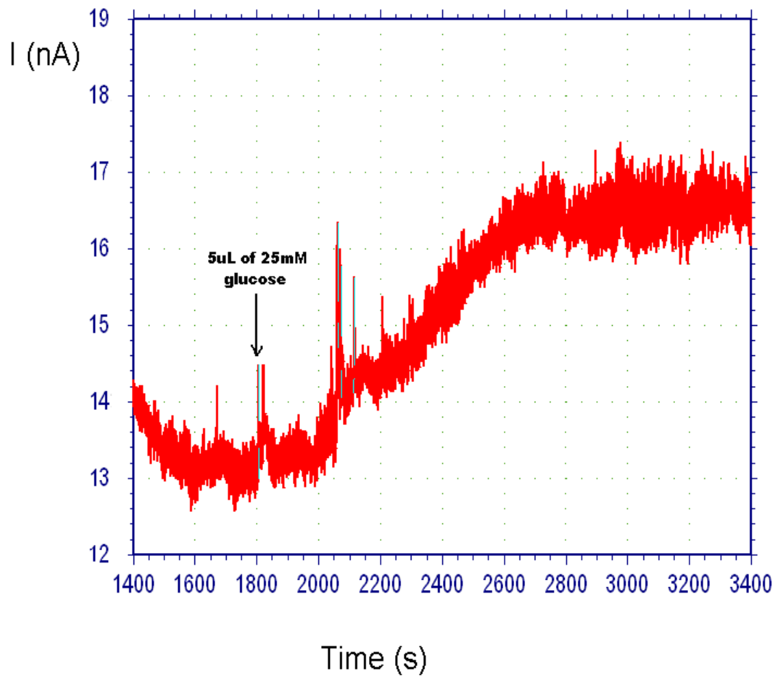
Figure 25: In-vivo Current Response of 176µm Pt/PPy/GOx sensor after injecting 0.125 mM of glucose. (5µL of 25mM solution of glucose)
