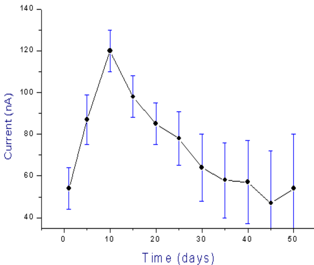
Figure 16: Long term stability of 176 \mu\text{m} glucose sensors with response to 5mM glucose in PBS solution (pH7.4). Working potential: +0.6V (vs. Ag/AgCl) (n=3)
