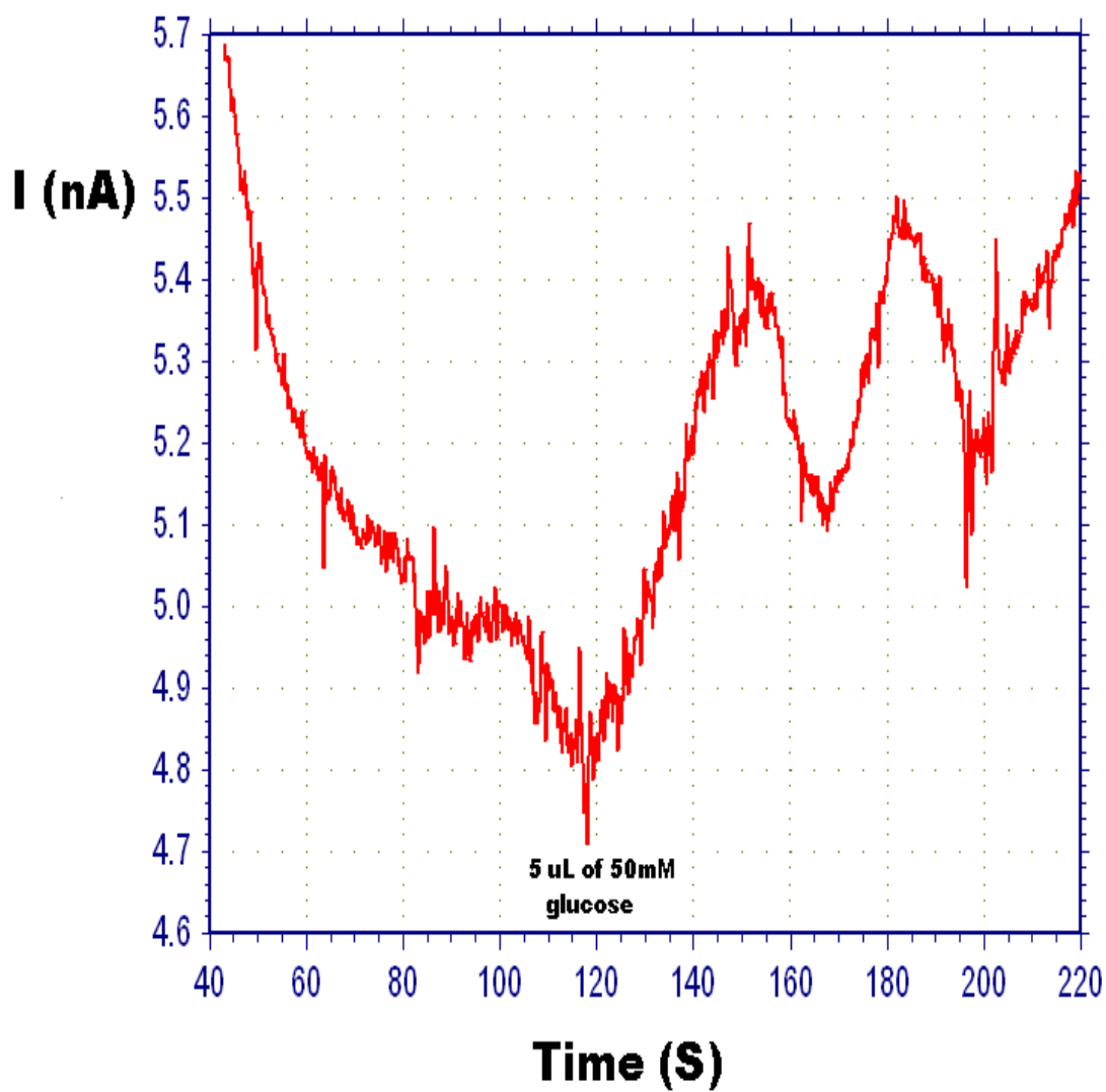
Figure 24: In-vivo Current Response of 25µm Pt/PPy/GOx sensor after injecting 0.25 mM glucose. (5µL of 50mM solution of glucose) Initially, the sensor had a decreasing background current and after the glucose was injected the current signal was increased. Then, the current signal was fluctuated between 5.5 -5.1nA.
