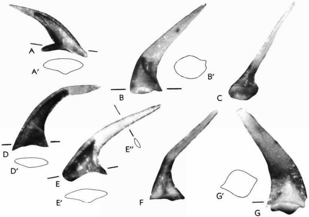
Fig. 3. Elements of three genera, illustrating shape of basal cavity and distribution of white matter—A. Cambrooistodus cambricus (Miller); lateral view and transverse section of compressed element from San Saba Member of Wilberns Formation, Llano uplift, Texas; 415 m (1,360 ft) above base of Threadgill Creek section of Barnes and Bell (1977), X55, USNM 303420.—B, C, F, G. Utahconus utahensis (Miller) from Signal Mountain Limestone, Wichita Mountains, Oklahoma, 530 m (1,735 ft) above base of measured section of Stitt (1977); lateral view (B) with transverse section (B'), and posterior view (C) of unicostate element, X110, USNM 303431; lateral (F) and posterior views (G) with transverse section (G') of bicostate element, X110, USNM 303430.—D, E. Eoconodontus notchpeakensis (Miller) from same formation and horizon as A; lateral views with transverse sections of rounded element (D, D') USNM 303416, and compressed element (E, E'), USNM 303417; both X110.
