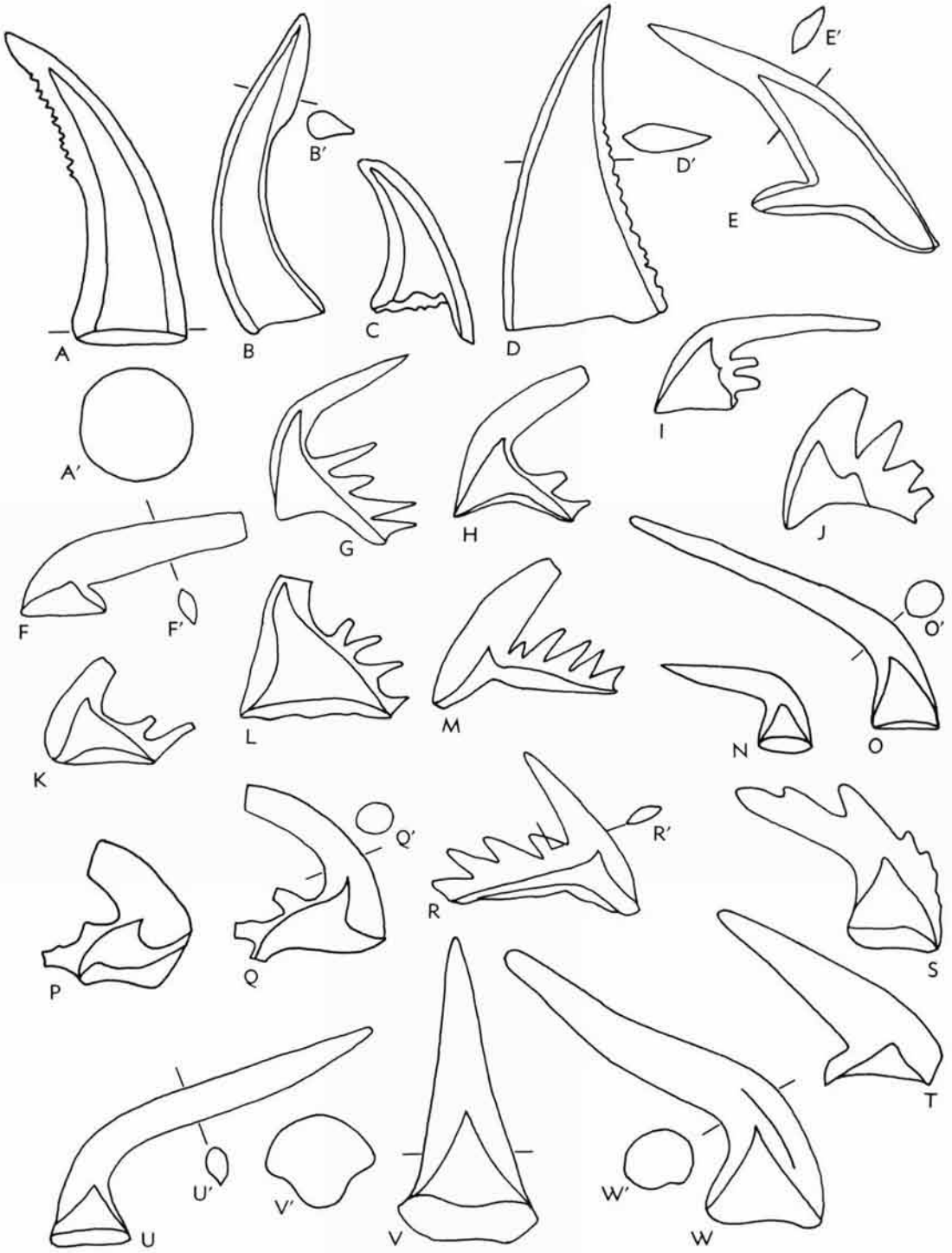
Fig. 4. Outlines of various conodont elements showing shapes of basal cavities and, for some, transverse sections (prime letters)—A. Proconodontus tenuiserratus , n. sp. (holotype, Pl. 1, fig. 2).—B. Proconodontus posterocostatus , n.
