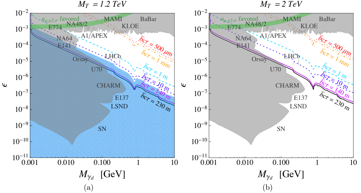
Figure 6.10: Various decay lengths of the dark photon originating from VLQs with masses (a) 1.2 TeV and (b) 2 TeV in \varepsilon - M_{\gamma_d} plane. The blue shaded regions are excluded by searches for stop pair production with decay \tilde{t} \rightarrow t \tilde{\chi}_1^0 . Gray shaded regions correspond to existing 90% confidence level limits from the SLAC and Fermilab beam dump experiments E137, E141, and E774 [200, 294, 295, 296], the U70 accelerator [297, 298], LHCb [299, 300], NA64 [301], the electron and muon anomalous magnetic moment a_\mu [302, 202, 303], KLOE [304, 305], WASA-at-COSY [306], the test run results reported by APEX [307] and MAMI [308], an estimate using a BaBar result [200, 309, 310], and a constraint from supernova cooling [311, 312]. The shaded green regions are favored to explain the muon anomalous magnetic moment [302] at 95% confidence level.
