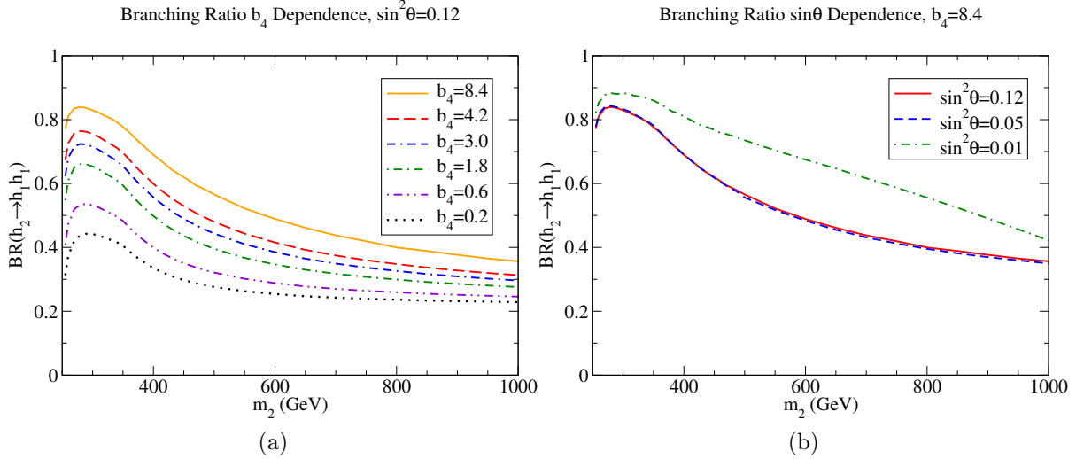
Figure 2.4: Maximum allowed \text{BR}(h_2 \rightarrow h_1 h_1) as a function of m_2 for different values of (a) b_4 and (b) \sin^2 \theta .
