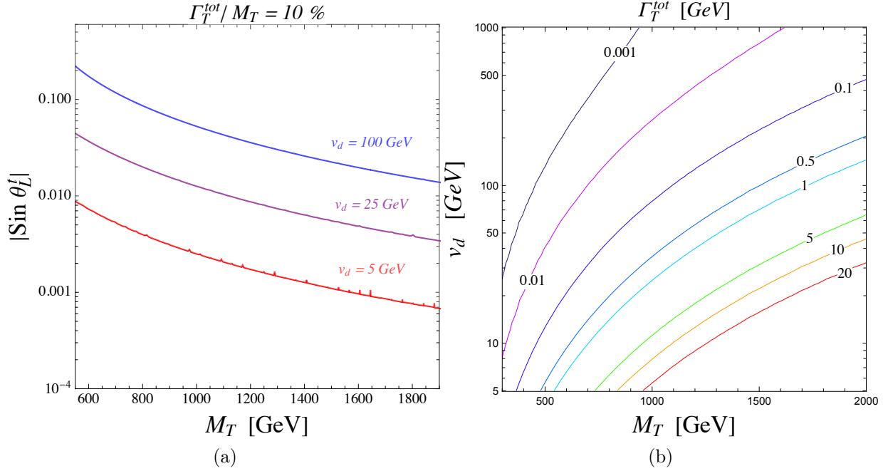
Figure 6.7: (a) Contours of \Gamma_T^{tot}/M_T = 0.1 in the M_T - \sin \theta_L^t plane for various v_d . (b) The total width ( \Gamma_T^{tot} ) of T in M_T - v_d plane for \sin \theta_L^t = 0.001 . For both sub-figures, we set \varepsilon = 0.001 , M_{\gamma_d} = M_2 = 2 GeV, and \sin \theta_S to its maximal value in Eq. (6.50).
