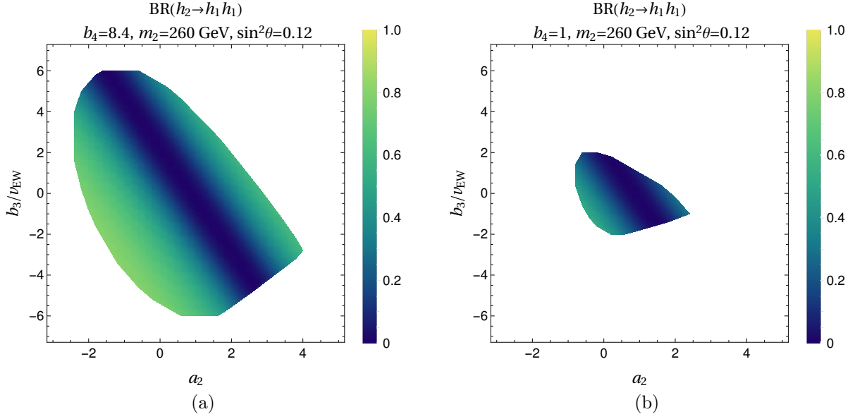
Figure 2.1: \text{BR}(h_2 \rightarrow h_1 h_1) as a function of b_3 and a_2 for m_2 = 260 \text{ GeV} and \sin^2 \theta = 0.12 . In (a) b_4 = 8.4 and (b) b_4 = 1 . The shaded regions are allowed by the global minimum and vacuum stability constraints. The color indicates \text{BR}(h_2 \rightarrow h_1 h_1) .
