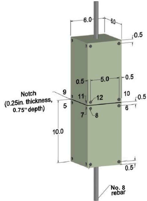
Figure 3.11: Tension Specimen Source: Tameemi and Lequesne (2015)
