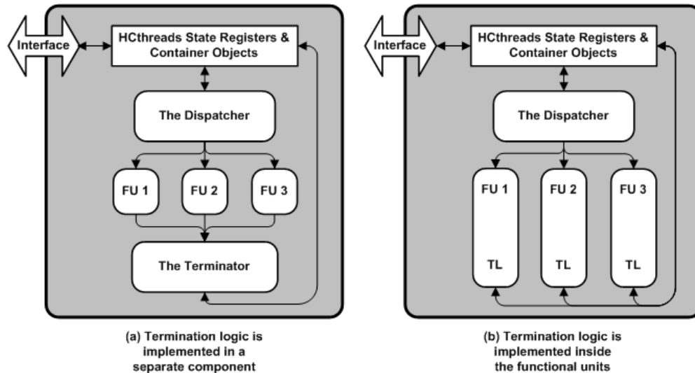
Figure 5.1. HCthreads internals assuming three functional units
