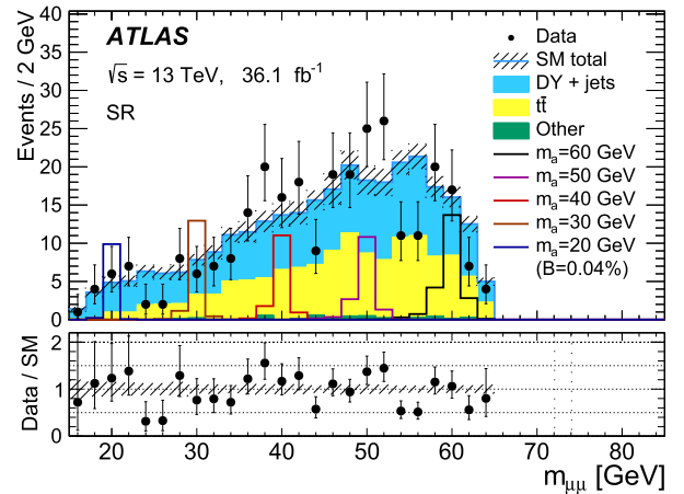
Fig. 5. The predicted and observed m_{\mu\mu} distributions in the SR after the background-only fit. The signal distributions are also shown assuming the SM Higgs boson cross-section (including ggF, VBF and VH production) and \mathcal{B}(H \rightarrow aa \rightarrow bb\mu\mu) = 0.04\% . The hashed bands show the total statistical and systematic uncertainties of the backgrounds.
