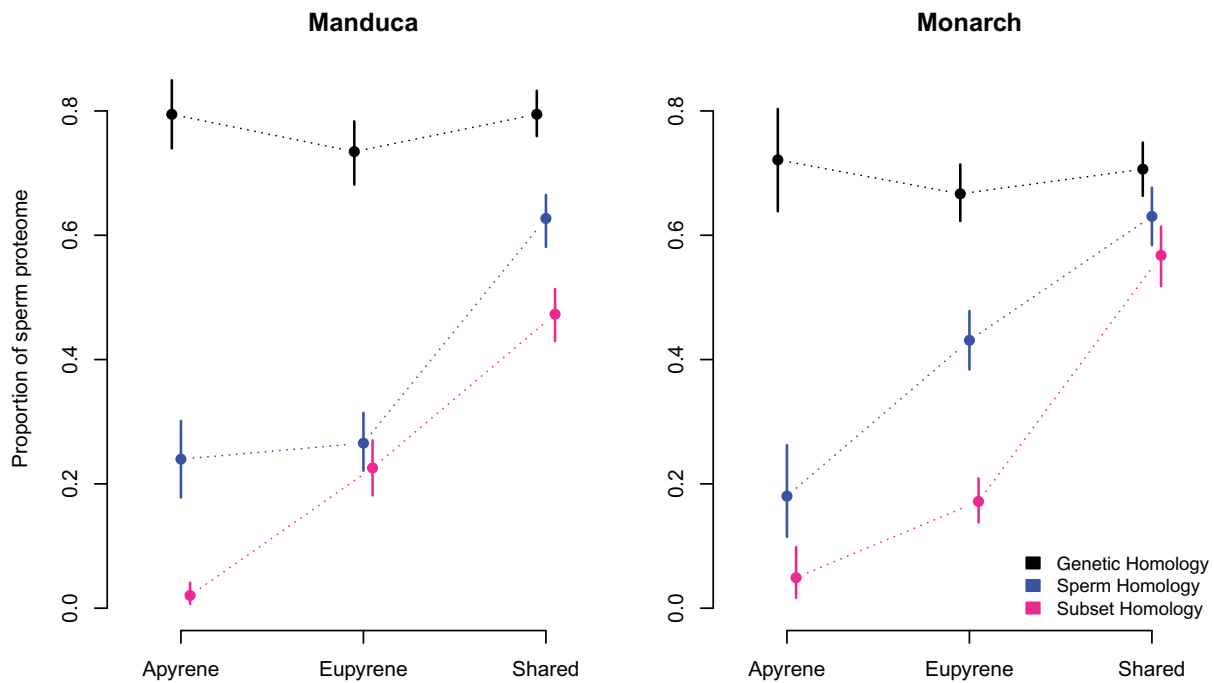
Fig. 3. —Proportions of proteins homologous between monarch and Manduca in each subset of the sperm proteome. The proportion of homologs are plotted for each subset of the sperm proteome: apyrene-specific, eupyrene-specific, and shared. Three different, increasingly stringent, criteria for homology are displayed. Genetic homology (black) indicates predicted orthologs found in the genomes of both species. Sperm homology (blue) indicates predicted orthologs found in the sperm of both species, regardless of sperm morph. Subset homology (magenta) indicates sperm homologs found in the same subset of the sperm proteome in both species.
