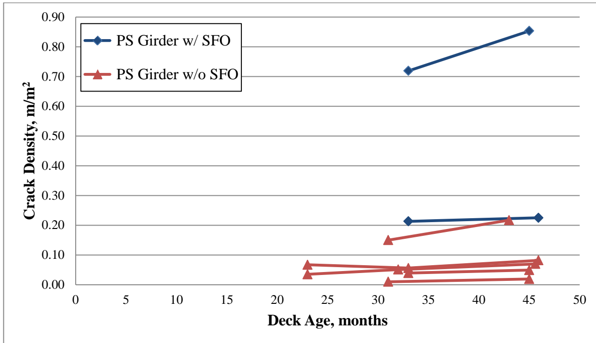
Figure 33: Crack Density versus age for decks with and without silica fume overlays (SFO) supported by prestressed (PS) girders
