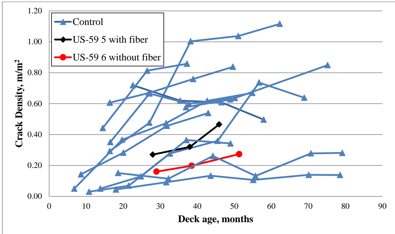
Figure 37: Crack density versus age for control (from LC-HPC study) and US-59 decks with silica fume overlays supported by steel girders
