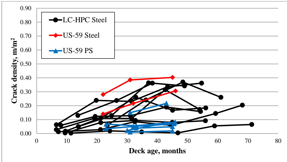
Figure 32: Crack density versus age for LC-HPC and US-59 monolithic decks supported by steel girders compared to US-59 monolithic decks supported by prestressed (PS) girders
