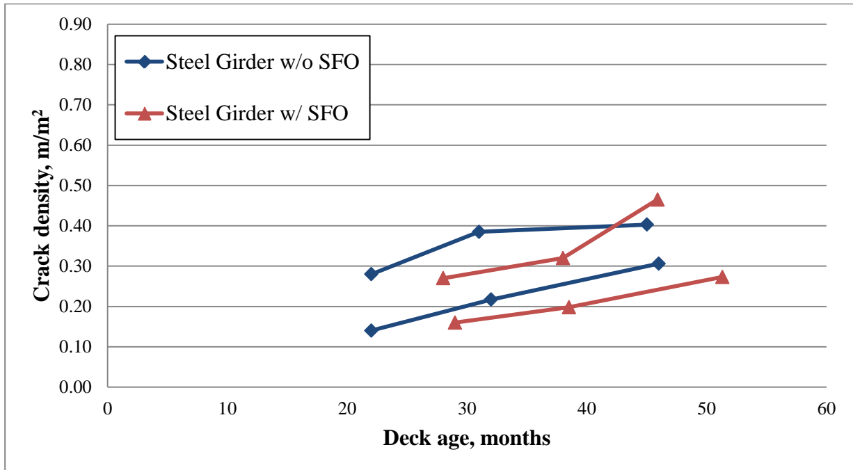
Figure 34: Crack Density versus age for decks and decks with and without silica fume overlays (SFO) supported by steel girders
