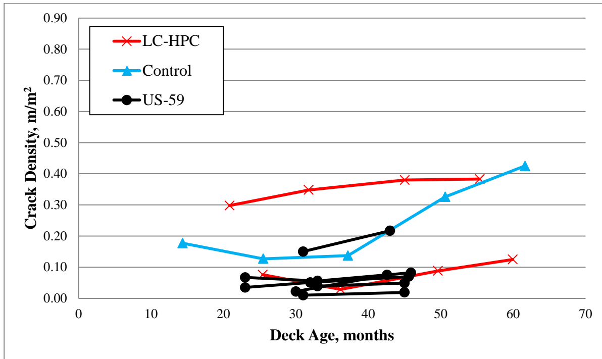
Figure 36: Crack density versus age for LC-HPC, control, and US-59 monolithic decks supported by prestressed girders
