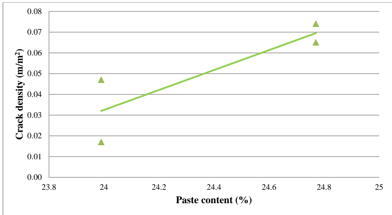
Figure 40: Crack density at 42 days versus paste content for US-59 decks prestressed girders with deck panels
