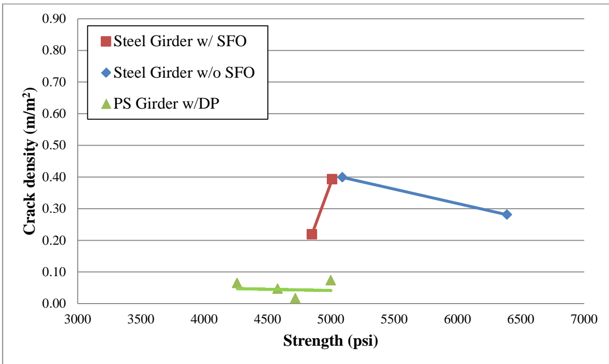
Figure 39: Crack density versus strength for US-59 decks supported by steel and prestressed girders constructed by Ames
