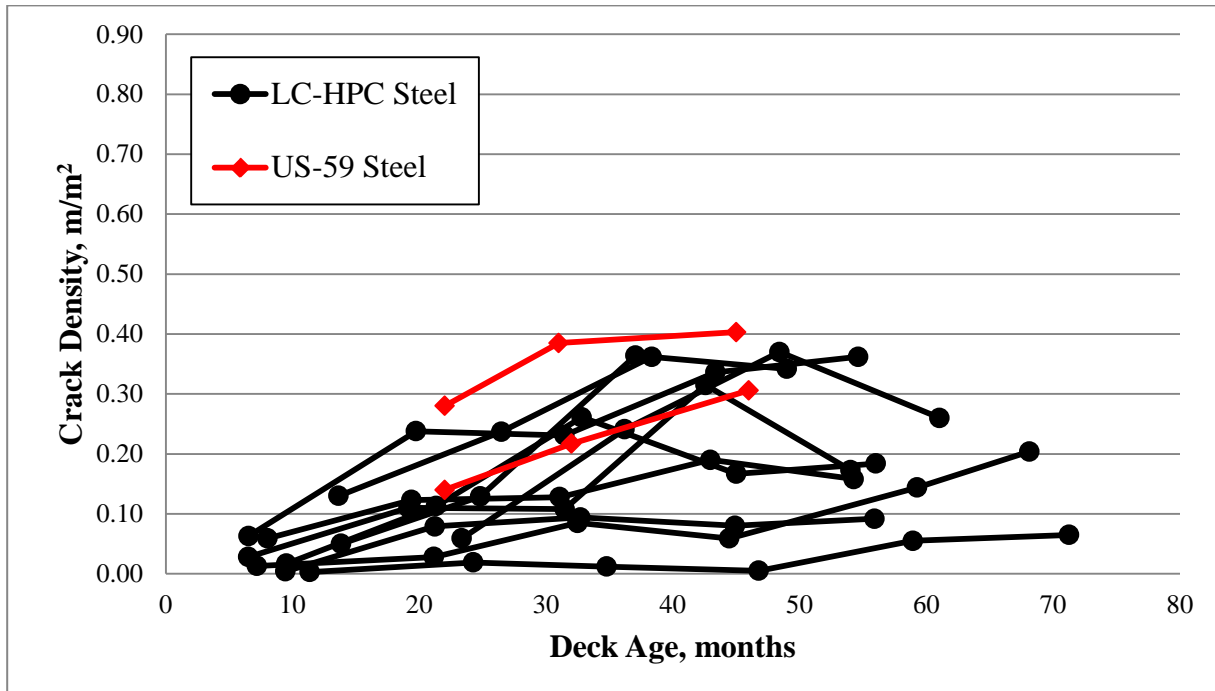
Figure 35: Crack density for age for LC-HPC and US-59 monolithic decks supported by steel girders
