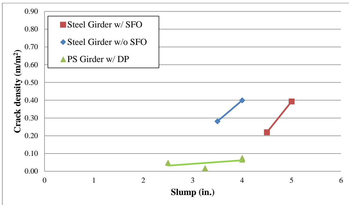
Figure 38: Crack density at 42 months versus slump for US-59 decks supported by steel and prestressed girders constructed by Ames
