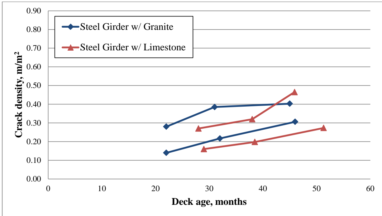
Figure 42: Crack density versus age of deck for US-59 decks supported on steel girder
