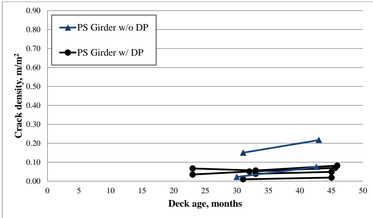
Figure 31: Crack density versus age for US-59 decks supported by prestressed girders with and without deck panels (DP)
