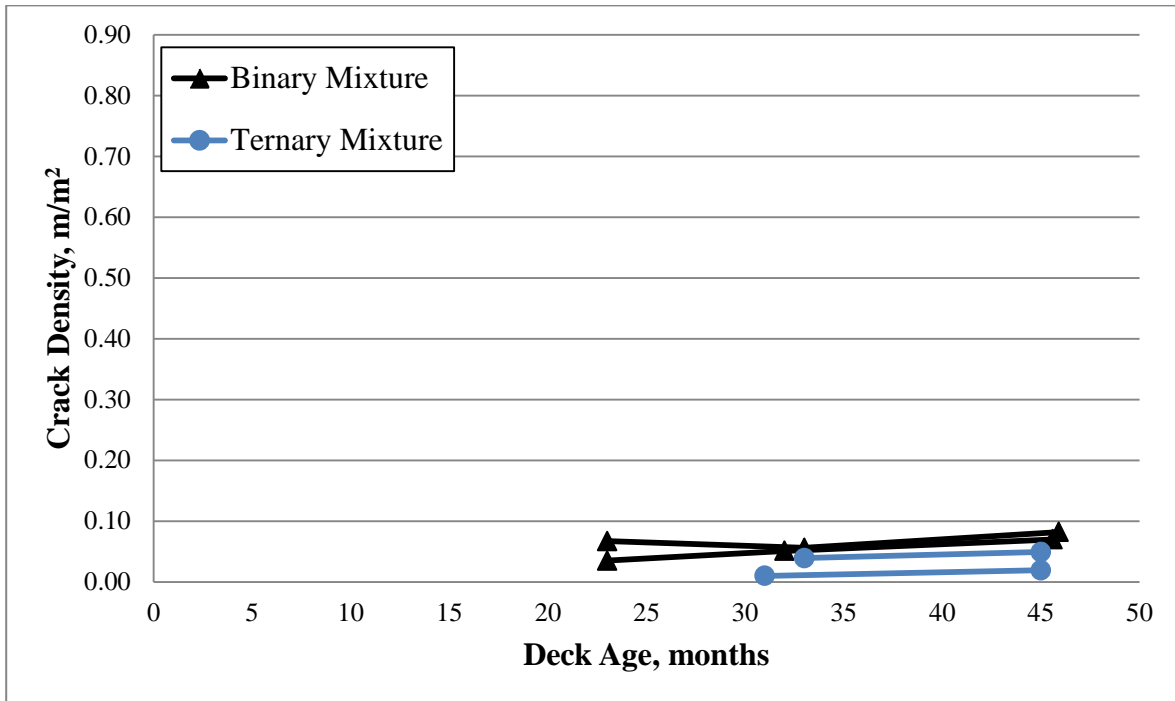
Figure 41: Crack density versus age for US-59 decks with deck panels supported prestressed girders with different cementitious material.
