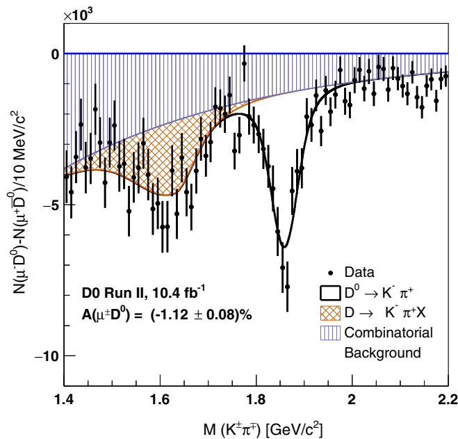
FIG. 2. The results of a fit to the differences between the numbers of \mu^-D^0 and \mu^+\bar{D}^0 events as function of the K\pi mass.
