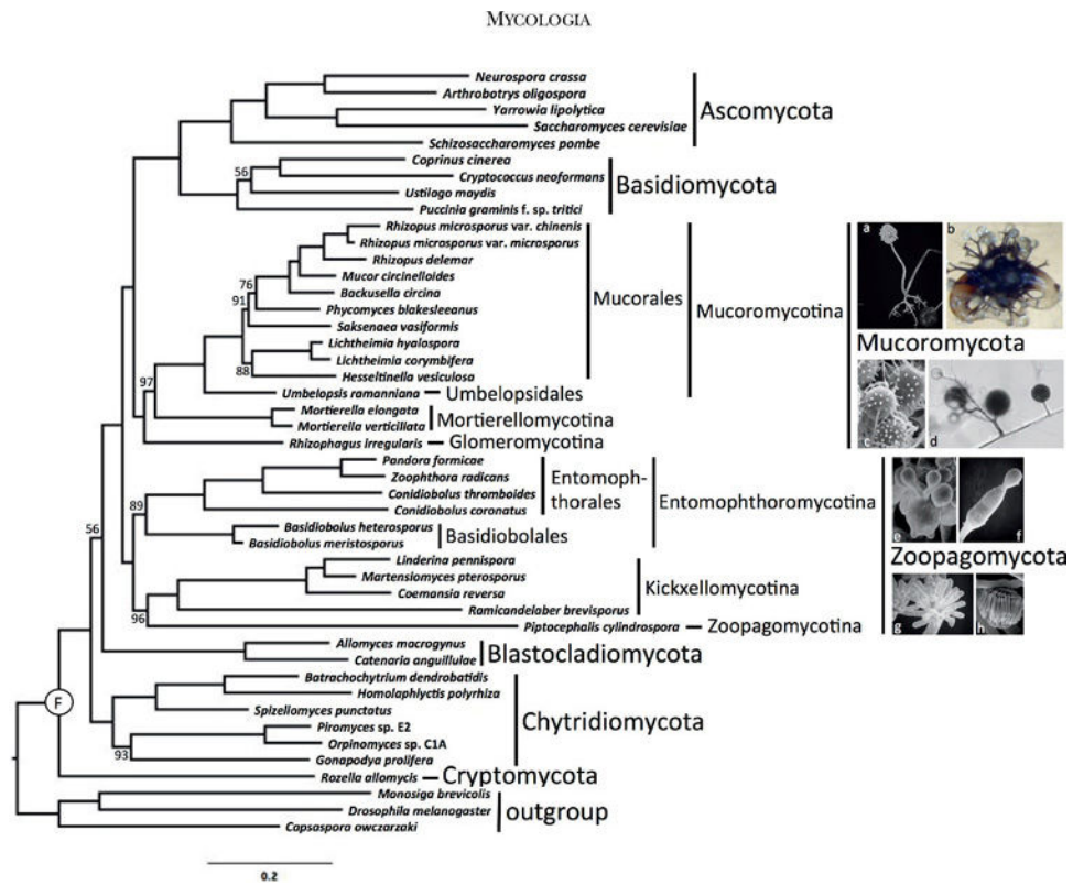
FIG. 1. RAxML phylogenetic tree of Kingdom Fungi based on the concatenated alignment of 192 conserved orthologous proteins. All branches received 100% bootstrap partitions except where noted by number above or below respective branches. Example images include: a. Rhizopus sporangium (SEM). b. Phycomyces zygospore (LM). c. Mortierella chlamydospores (SEM). d. Rhizophagus spores and hyphae (LM). e. Conidiobolus secondary (replicative) conidia forming on primary conidium (SEM). f. Basidiobolus ballistosporic conidium (SEM). g. Piptocephalis merosporangia (SEM). h. Linderina merosporangium (SEM). LM: light micrograph, SEM: scanning electron micrograph.
