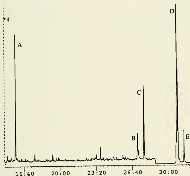
Fig. 2. Chromatogram of the derivatized (with BSTFA) reaction of Triepolus distinctus glandular pouches. Peak "A" = unidentified, two active hydrogen groups, two oxygens, and a molecular weight of 259. Peak "B" = C_{16} fatty acid. Peak "C" = a long-chain fatty acid TMS ester. Peak "D" = monounsaturated C_{18} fatty acid TMS ester. Peak "E" = a saturated stearic acid TMS ester. Peaks "A," "B," and "C" are magnified times four.
