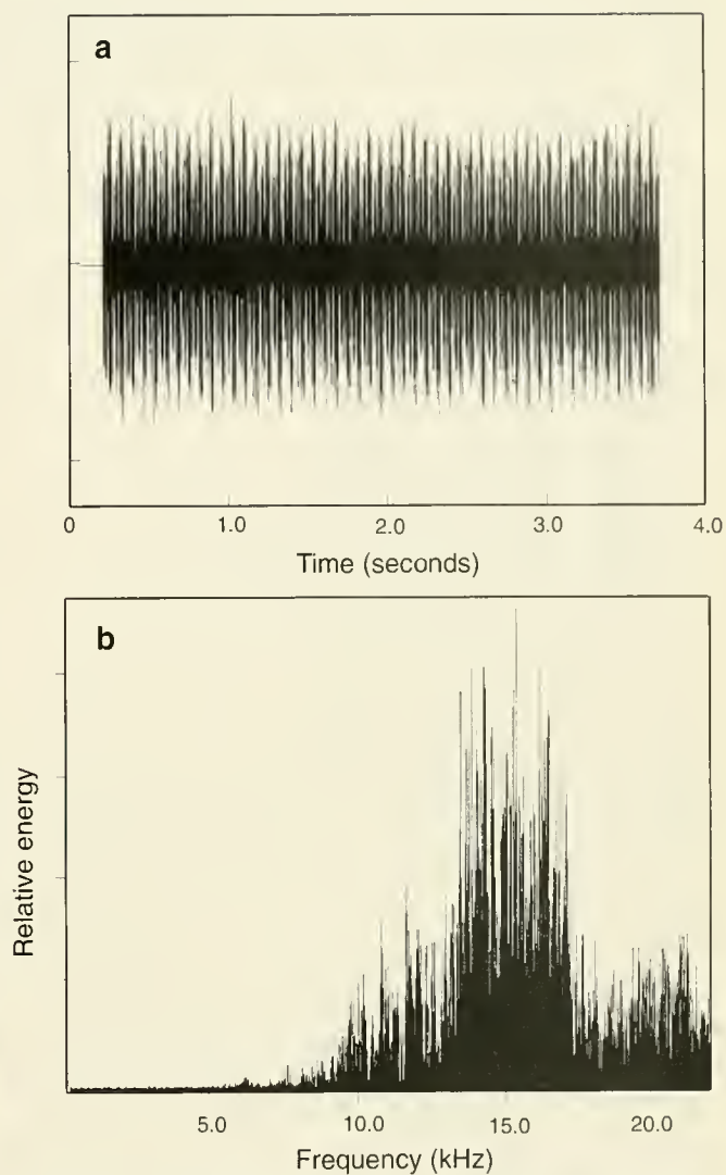
Fig. 3. Calling song of male Neoconocephalus affinis ; (a) oscillogram, (b) frequency spectrogram. The y-axis is scaled linearly in both (a) and (b). See methods section for equipment used.
