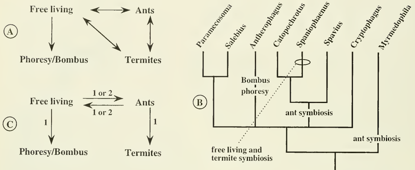
Fig. 5. Newly constructed character state transformations and phylogeny based on phoretic and nonphoretic symbiosis. A—Hypothetical character state graph. B—Phylogenetic reconstruction of the Cryptophagus group based on cladistic analysis that included character states in A. C—Character state graph based on reconstruction in B with number of transformations indicated at each transition.
