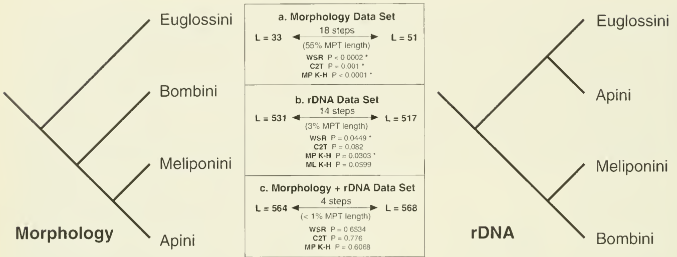
Fig. 4. Statistical tests of alternative hypotheses of tribal-level relationships in the corbiculate bees. WSR = Wilcoxon's signed-rank test, C2T = Compare 2 trees test, MP K-H = parsimony-based Kishino-Hasegawa parametric test, ML K-H = likelihood-based Kishino-Hasegawa parametric test. (Left) the single most-parsimonious tree (MPT) resulting from unweighted parsimony analysis of the morphology data set. (Right) The MPT resulting from unweighted parsimony analysis of the rDNA data set. Asterisks (*) indicate significant power to distinguish between the alternative hypotheses at the 95% level. See text for description of tests. The ability of the morphology data set to distinguish between the two topologies is significant near the limits of resolution for all three tests, whereas the ability of the molecular data set to distinguish between the two topologies is non-significant at the 95% confidence level in two out of four tests. The combined data set is unable to distinguish between the two topologies by any of the three test criteria, indicating serious erosion of character support for tribal-level groupings due to the union of two significantly conflicting data sets. (Note that neither topology represents the most parsimonious solution for the combined data set.)
