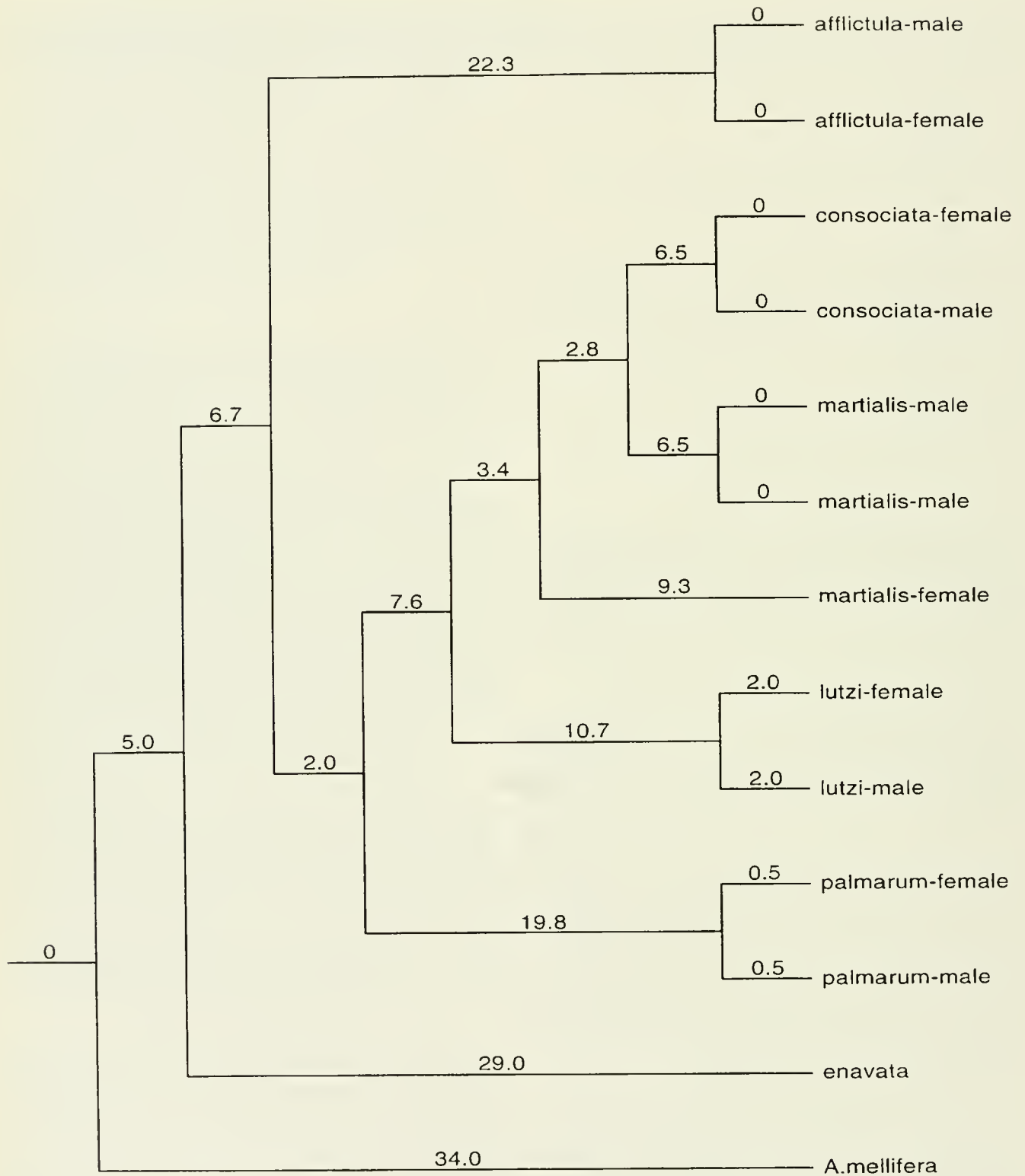
Fig. 1. UPGMA phenogram based on the matrix of absolute distances in Table 2. Numbers on phenogram are branch lengths. The phenogram does not necessarily reflect phylogenetic relationships among the species.
