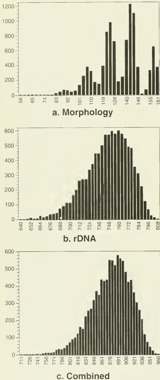
Fig. 2. The distribution of tree lengths (DTL's) for the morphology data set, the 16s rDNA data set, and for the data set produced by their combination, based on 10,000 trees generated by the "random trees" command in PAUP 3.1 (Swofford, 1991) (see text). Number of trees is indicated on the y-axis, tree length on the x-axis. Hillis (1991) and Huelsenbeck (1991) have suggested that left-skewness, which is obvious in these three DTL's, indicates that the data contain strong phylogenetic signal.
