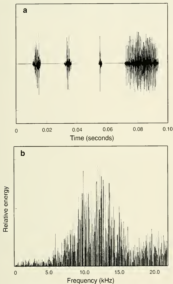
Fig. 2. Calling song of male Orophus conspersus ; (a) oscillogram, (b) frequency spectrogram. The y-axis is scaled linearly in both (a) and (b). Refer to methods section for equipment.
