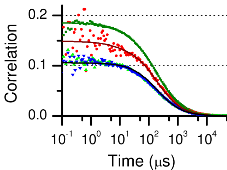
Figure 2. Correlation functions for polyproline-AF488-Atto 740: G_{GG}(\tau) (green squares), G_{RR}(\tau) (red circles), G_{GR}(\tau) (green triangles), and G_{RG}(\tau) (blue inverted triangles). The solid lines show a global fit where the transit times for G_{GG}(\tau) , G_{GR}(\tau) , and G_{RG}(\tau) were linked (see text) and the initial amplitudes were allowed to vary independently. Fitting parameters are in Table 1.
