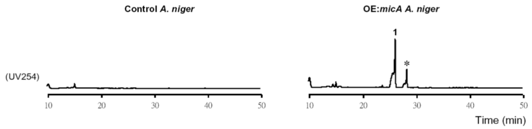
Fig. 3. LC-DAD-MS Analysis of wild-Type A. niger and amylase(p)-micA (OE: micA ) mutant metabolites. *A related compound that has similar MS/MS fragmentation with microperfuraneone.
