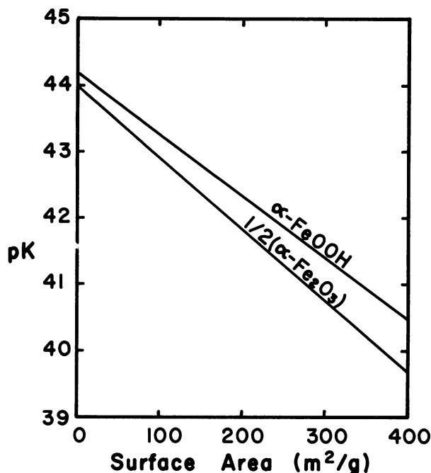
FIGURE 5. Effect of specific surface area on pK of goethite ( \alpha -FeOOH) and hematite ( 1/2 \alpha -Fe 2 O 3 ).
