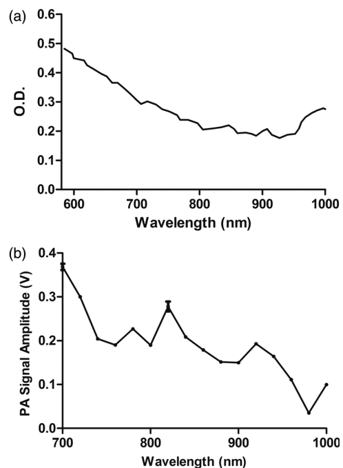
Fig. 3 Optical characteristics of DNDs suspended in DI water as a function of wavelength. (a) Absorption spectrum measured with an integrating sphere, and (b) photoacoustic (PA) spectrum.
