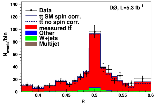
FIG. 1 (color online). The distribution of the discriminant R for \ell + jets events with four jets and an invariant mass of the two light-flavor jets within \pm 25 GeV of the mass of the W boson. The expectation (including background) for complete spin correlation as predicted by the SM ( f = 1 ) and the case of no spin correlation ( f = 0 ), as well as the t\bar{t} contribution for f_{\text{meas}} , where f_{\text{meas}} was taken from the combined fit in the \ell + jets and dilepton final states, are shown. The first and last bins include contributions from R < 0.37 and R > 0.60 , respectively. The bin width is chosen to minimize the statistical uncertainty.
