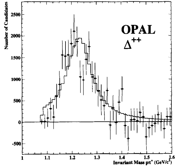
Fig. 3. The \Delta^{++} candidate invariant mass spectra for all bins of x_E , after subtraction of the fitted background. The line shows the fitted \Delta^{++} contribution.
