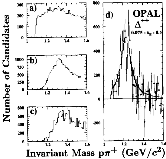
Fig. 2. Some of the background shapes that make up the fit to the second x_E bin ( 0.075 < x_E < 0.1 ). a) The fitted prediction for the p\pi^+ component, without the \Delta^{++} . b) The fitted prediction for the \pi^+\pi^+ component. c) The fitted prediction for the \pi^+p component. d) The resulting spectrum after the fitted background has been subtracted with the fitted \Delta^{++} contribution shown.
