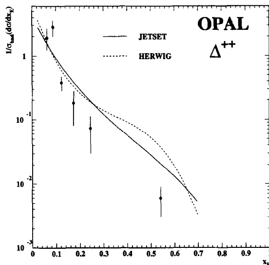
Fig. 4. The \Delta^{++} fragmentation function as a function of x_E . The points are the measurements, the solid line is the prediction of JETSET and the dashed line is the prediction of HERWIG. The data points have been plotted at the values of x_E inferred from JETSET, given in table 4, following the prescription in [17]. The Monte Carlo predictions are normalised to the observed rates above x_E of 0.05.
