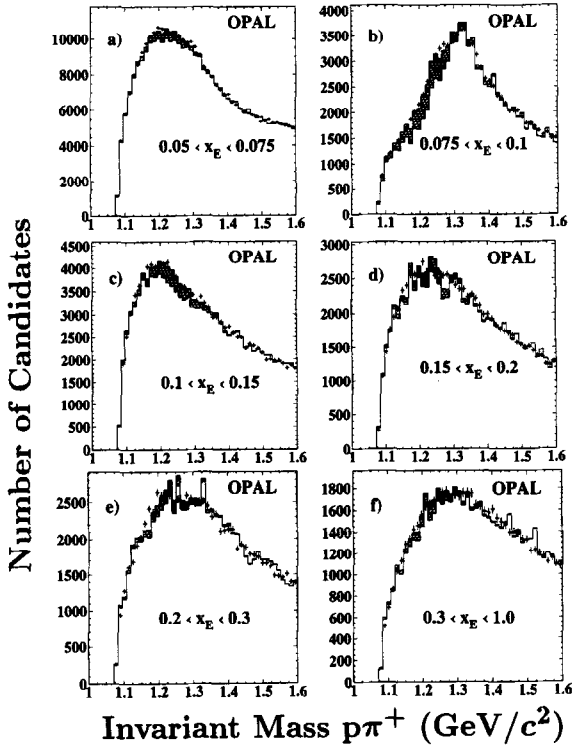
Fig. 1. The \Delta^{++} candidate invariant mass spectra along with the results of the fit. The open histogram is the fitted background shape and the shaded histogram shows the fitted \Delta^{++} signal. The x_E bins are: a) 0.05 < x_E < 0.075 , b) 0.075 < x_E < 0.1 , c) 0.1 < x_E < 0.15 , d) 0.15 < x_E < 0.2 , e) 0.2 < x_E < 0.3 , f) 0.3 < x_E < 1.0 .
