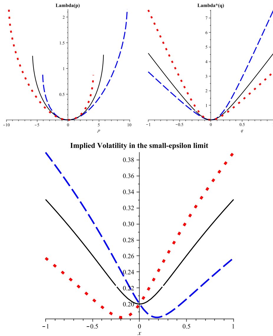
Figure 1. Here we have plotted \Lambda , \Lambda^* , and the implied volatility in the small- \epsilon limit as a function of the log-moneyness x = \log(K/S_0) . The parameters are t = 1 , ergodic mean \theta = .04 , convexity \nu/\kappa = 1.74 ( \kappa = 1.15 , \nu = .2 ), and skew \rho = -.4 (dashed blue), \rho = 0 (solid black), \rho = +.4 (dotted red).
