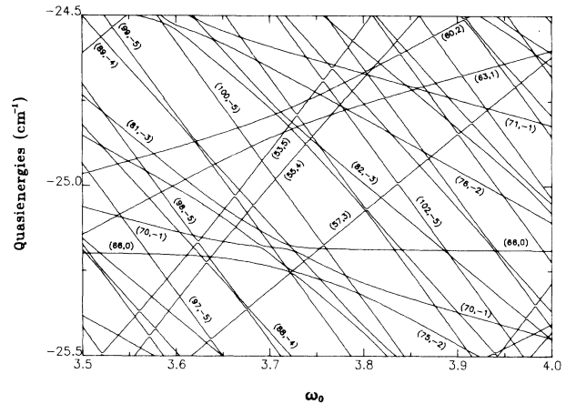
FIG. 4. Same as Fig. 3 except for \omega_0 near region E ( \omega_0 \sim 3.66 ), where multiphoton resonant transitions are significant. Quasi-energy-level avoided crossings are more isolated in this region, and the identities of quasienergy levels can be easily distinguished as shown.
