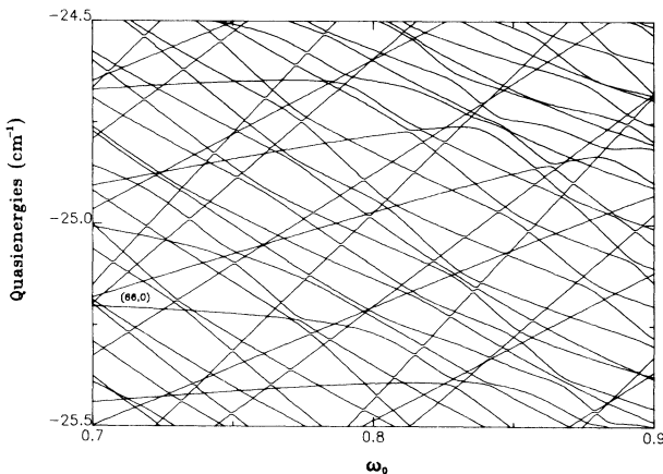
FIG. 3. Quasienergy avoided-crossing pattern near region B ( \omega_0 \sim 0.8 ) where quantum diffusion is the dominant excitation mechanism. Physical parameters same as Fig. 2. Only a small cross section (between -25.5 and -24.5 \text{cm}^{-1} ) of quasienergies is shown. Most quasienergy levels are strongly perturbed and mixed and lose their identities. Excitation is very efficient in this region.
