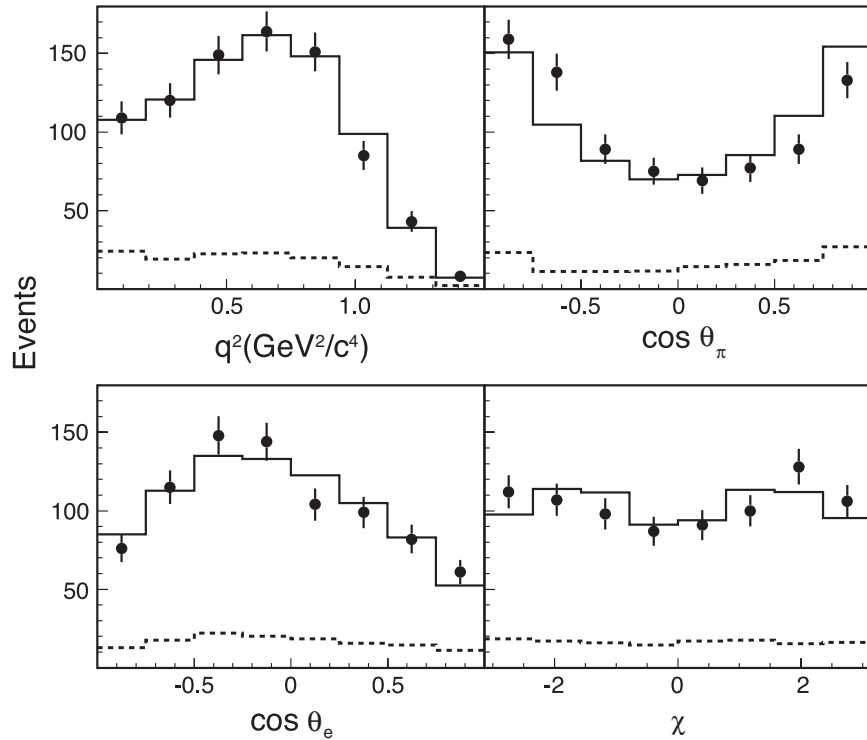
FIG. 2. Projections of the combined \rho^- and \rho^0 data (points with statistical error bars) and the fit (solid histogram) onto q^2 , \cos\theta_e , \cos\theta_\pi , and \chi . The dashed lines show the sum of the background distributions.
