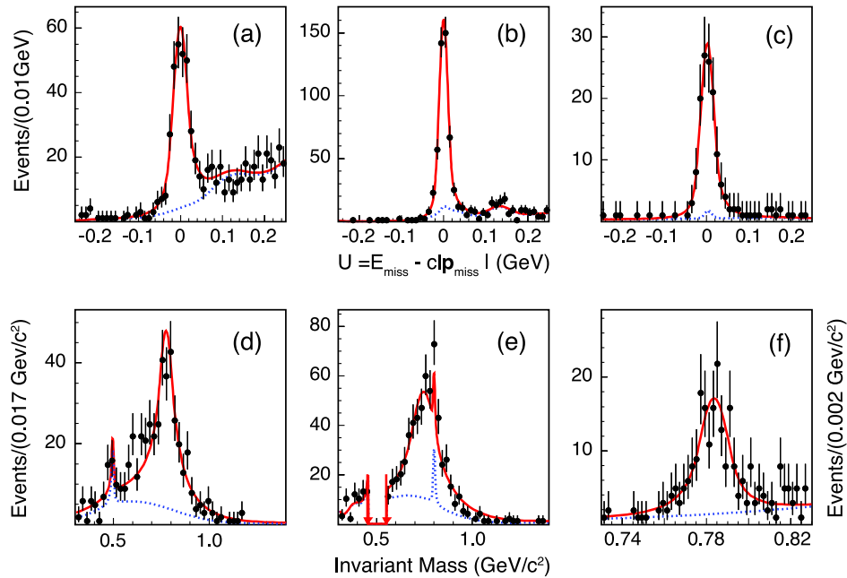
FIG. 1 (color online). Fits to the U and hadron invariant mass distributions in data (filled circles with error bars) for (a) and (d) D^0 \rightarrow \rho^- e^+ \nu_e , \rho^- \rightarrow \pi^-\pi^0 ; (b) and (e) D^+ \rightarrow \rho^0 e^+ \nu_e , \rho^0 \rightarrow \pi^+\pi^- ; and (c) and (f) D^+ \rightarrow \omega e^+ \nu_e , \omega \rightarrow \pi^+\pi^-\pi^0 . The solid line represents the fit of the sum of the signal function and background function to the data. The dashed line indicates the background contribution. The arrows indicate a \pm 48 \text{ MeV} region around the K_S^0 mass, which has been removed for display.
