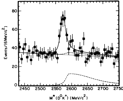
FIG. 2. Histogram of M^*(D^0 K^+) , with fit. The solid line shows the complete signal and background fitting functions. The sum of the background functions is shown by the dashed line. The dotted line shows just the polynomial used to represent the combinatoric background. The shape of the D_s^*(2470)^+ background function is shown at the bottom by the dash-dotted line, with the area scaled up by a factor of 5.
