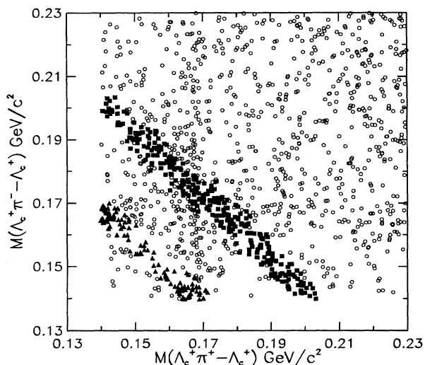
FIG. 2. Scatter plot of the mass difference M(\Lambda_c^+ \pi^-) - M(\Lambda_c^+) vs the mass difference M(\Lambda_c^+ \pi^+) - M(\Lambda_c^+) , for events with M(\Lambda_c^+ \pi^+ \pi^-) < 2650 \text{ MeV}/c^2 . Visible in the figure are (1) the vertical band at \Lambda_c^+ \pi^+ mass difference of 168 \text{ MeV}/c^2 , corresponding to \Sigma_c^{*+} \rightarrow \Lambda_c^+ \pi^+ ; (2) the horizontal band at \Lambda_c^+ \pi^- mass difference of 168 \text{ MeV}/c^2 , corresponding to \Sigma_c^0 \rightarrow \Lambda_c^+ \pi^- ; (3) the diagonal band extending from (0.14, 0.20) to (0.20, 0.14), corresponding to combinations taken from the \Lambda_c^{*+}(2625) signal region in Fig. 1 (squares); and (4) the diagonal band extending from (0.14, 0.168) to (0.168, 0.14), corresponding to combinations taken from the \Lambda_c^{*+}(2593) signal region in Fig. 1 (triangles), within which there are two lobes at the kinematic limits: (a) the enhancement in the \Sigma_c^{*+} band, just above the threshold for \Lambda_c^+ \pi^- , and (b) the enhancement in the \Sigma_c^0 band, just above the threshold for \Lambda_c^+ \pi^+ .
