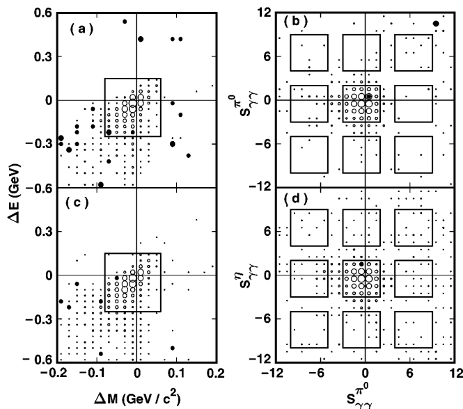
FIG. 1. (a) \Delta E vs \Delta M distribution of \tau^- \rightarrow \mu^- \pi^0 \pi^0 candidates with -12 < S_{\gamma\gamma} < 12 in the data and signal Monte Carlo (open circles) samples. (b) S_{\gamma\gamma}^{\pi^0} vs S_{\gamma\gamma} distribution for the center box in the \Delta E vs \Delta M plane. (c) and (d) are the corresponding distributions for \tau^- \rightarrow e^- \pi^0 \eta . The signal, sideband, and corner-band regions in the S_{\gamma\gamma} vs S_{\gamma\gamma} plane are indicated by the nine boxes. The size of the circles is proportional to the number of entries. The scale for the signal Monte Carlo event distributions is arbitrary.
