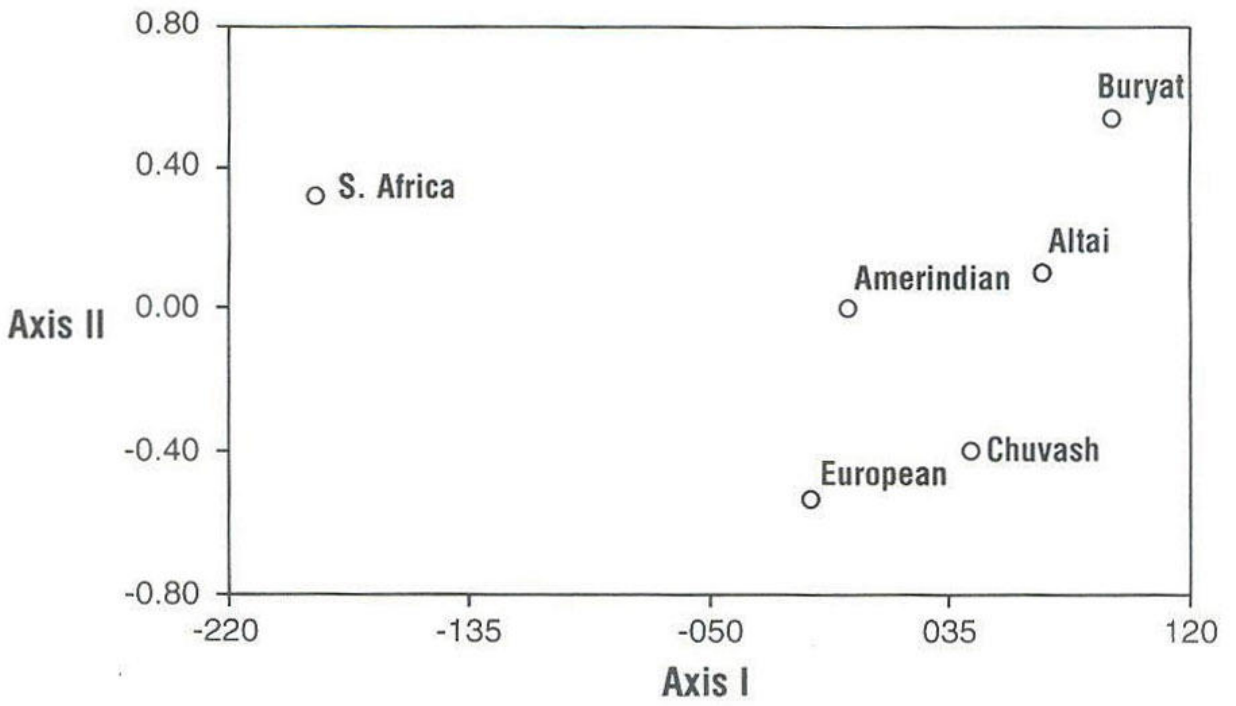
Figure 1. Two-dimensional scaling representation of genetic distances measured by R matrix and based on 296 loci and 2,203 alleles among 6 populations.
