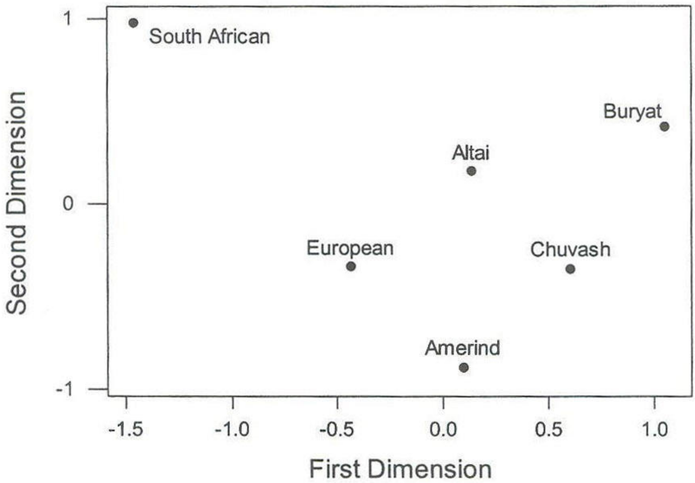
Figure 2. Two-dimensional scaling representation based on 30 randomly selected STR loci from the 6 populations characterized by DNA pools.
