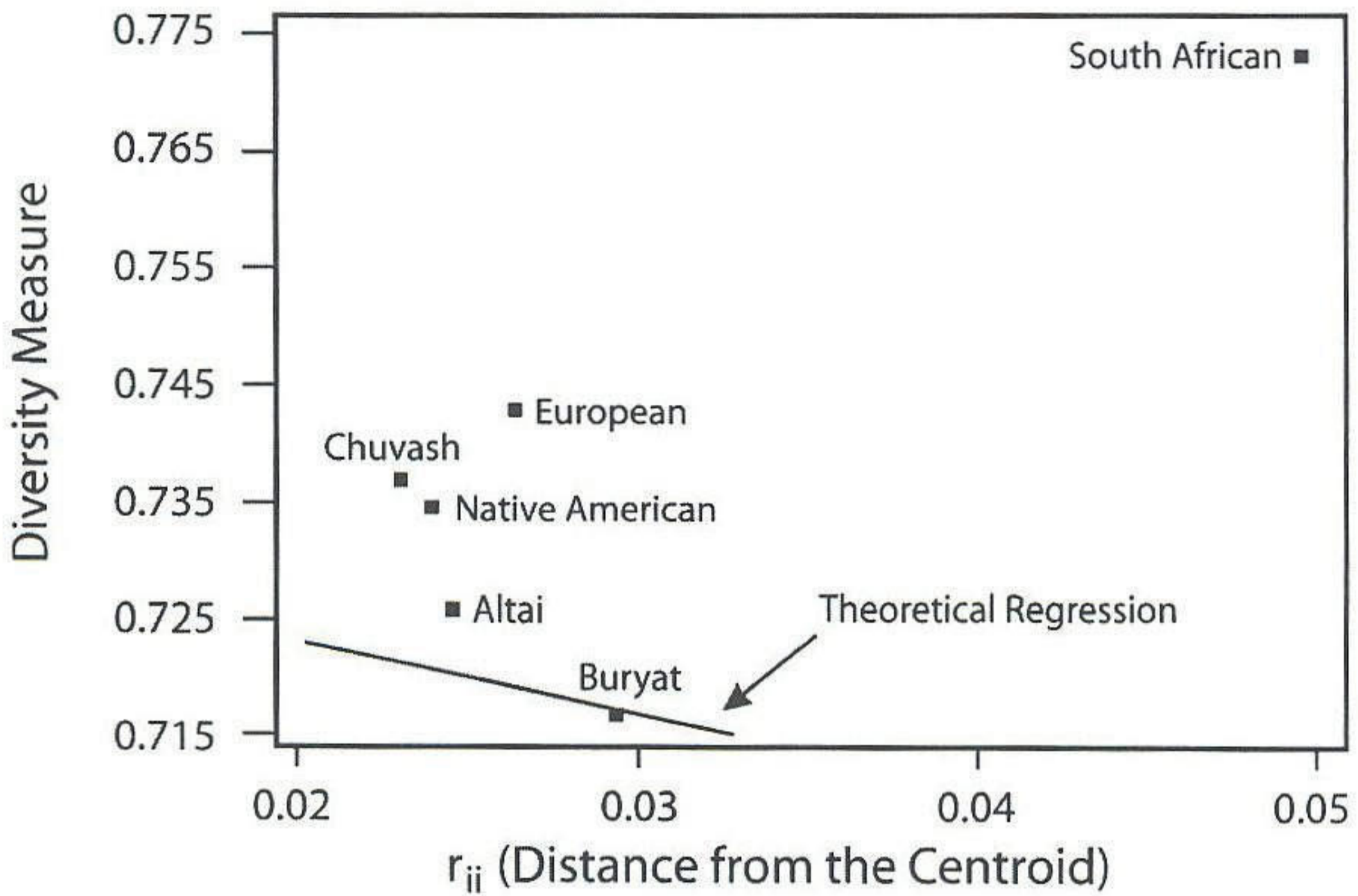
Figure 3. Plot of genetic diversity ( H ) against the distance from the centroid of distribution for 296 STR loci in 6 populations.
