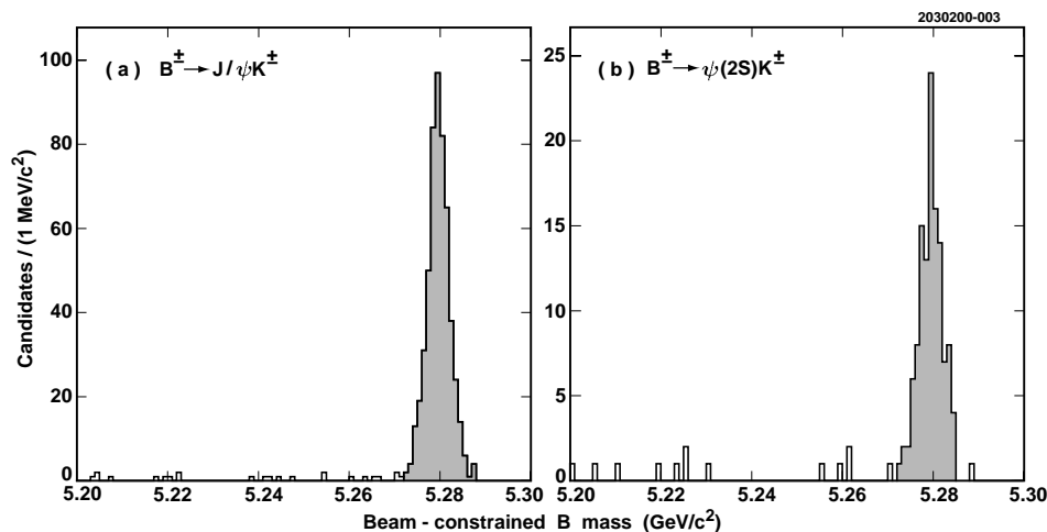
FIG. 2. Beam-constrained B mass distribution for (a) B^\pm \rightarrow J/\psi K^\pm and (b) B^\pm \rightarrow \psi(2S)K^\pm candidates passing the |\Delta E|/\sigma(\Delta E) < 3 requirement. The shaded parts of the histograms represent the 534 B^\pm \rightarrow J/\psi K^\pm and 120 B^\pm \rightarrow \psi(2S)K^\pm candidates that pass the |M(B) - M_B|/\sigma(M) < 3 requirement.
