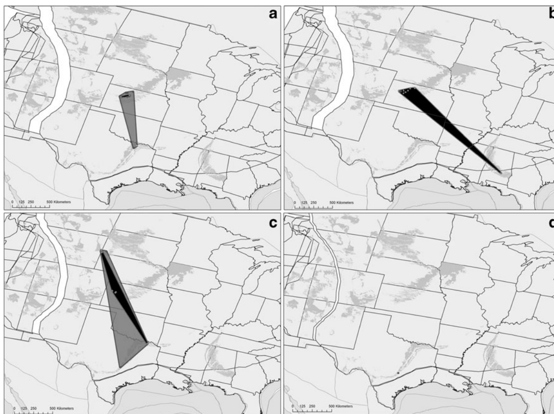
Fig. 2 Range reconstructions for marine vertebrate species from the Late Cretaceous showing how species distributions typically change through time. Darker polygons show the ranges of the mosasaur Tylosaur for different stages (a–d) of the Late Cretaceous. Lighter
