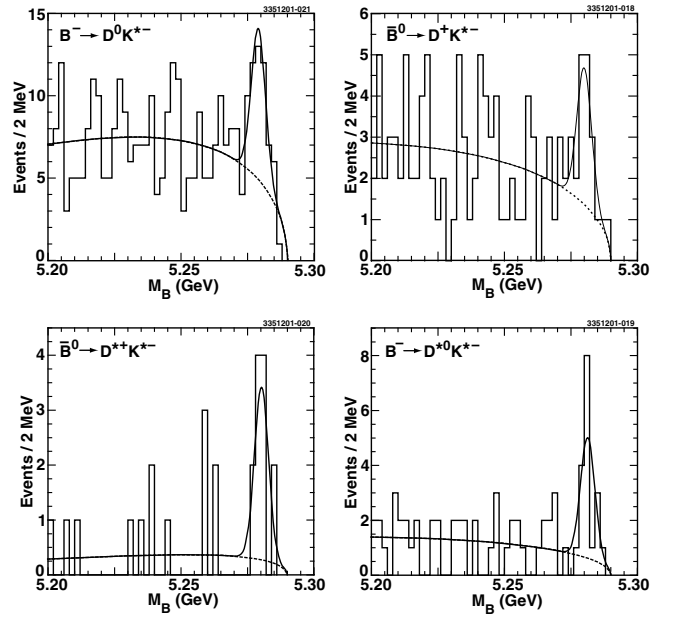
FIG. 1. The beam-constrained mass distributions for \bar{B} \rightarrow D^{(*)}K^{*-} decays (top left), with all submodes combined. The histograms show the data, the solid lines represent the overall fit to the data, and the dashed lines represent the fitted backgrounds under the peaks.
