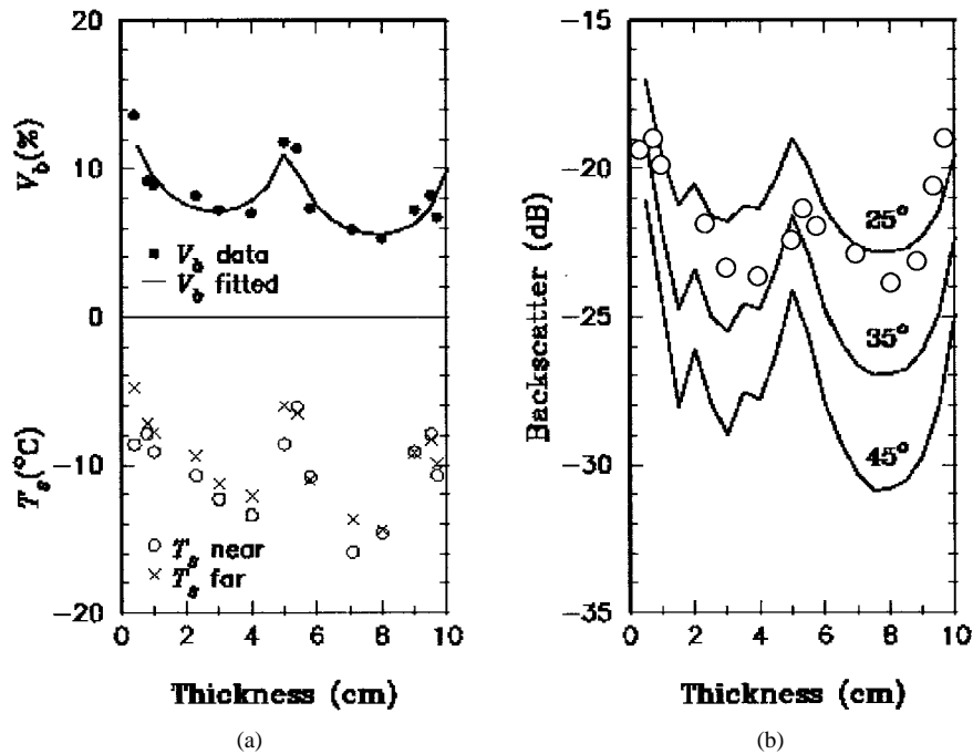
Fig. 8. (a) Sea ice surface temperature T_s measured near the area of the radar footprints and at the far side of the sea ice sheet, and the brine volume V_b corresponding to the temperature cycles. (b) Backscatter calculated at HH-polarization and 25, 35, and 45° incidence angles for the ice properties depicted in (a). Circles are measured HH-polarization backscatter data for 25° incidence [28].
