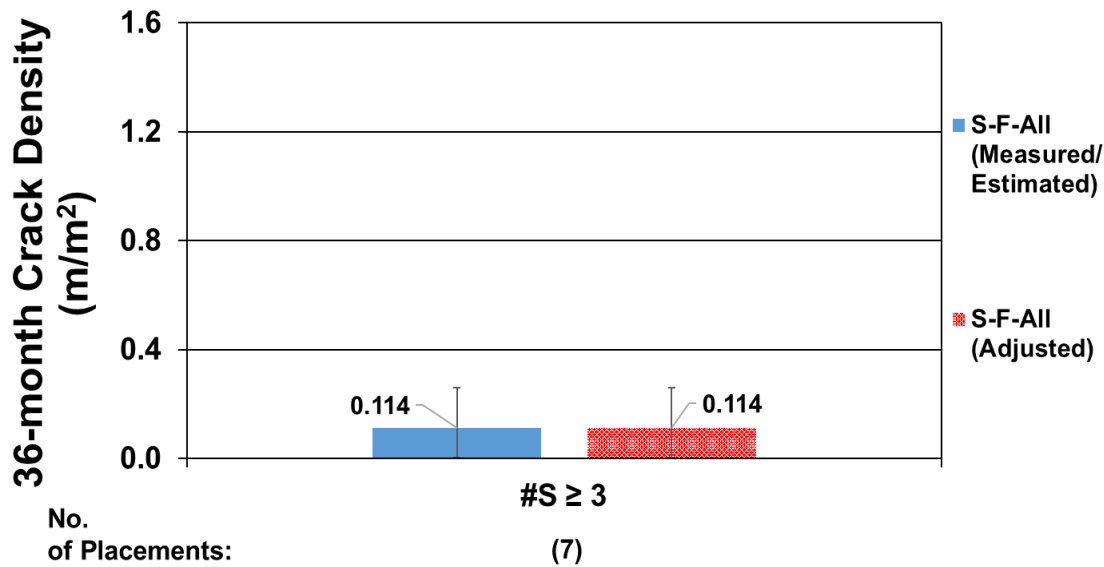
Figure E.20: Average measured/estimated and adjusted 36-month crack densities for all bridge decks supported by steel girders with fibers and different numbers of span (#S ≥ 3)
