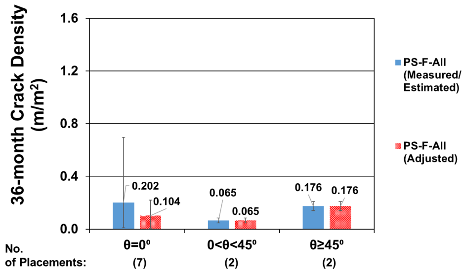
Figure E.4: Average measured/estimated and adjusted 36-month crack densities for all bridge decks supported by prestressed concrete girders with fibers and different skew
