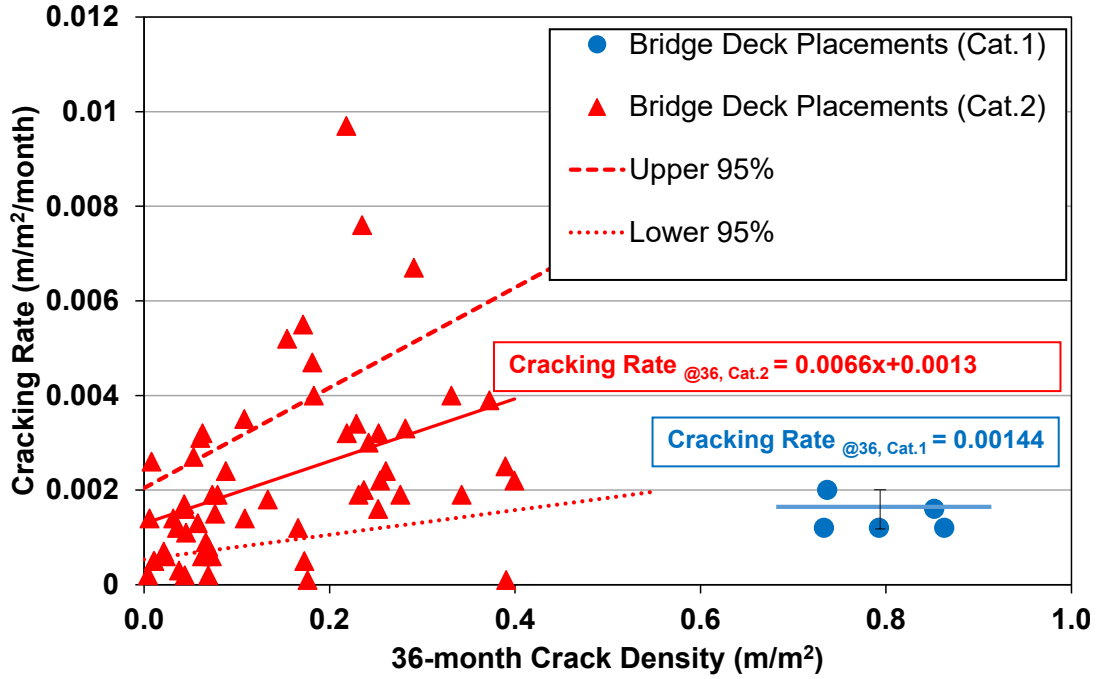
Figure C.3: Cracking rate as a function of 36-month crack density of the decks in Categories of 1 and 2
