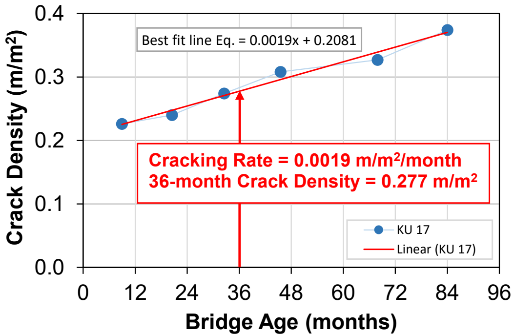
Figure C.1: Cracking Rate and 36-month crack density of LC-HPC 17
