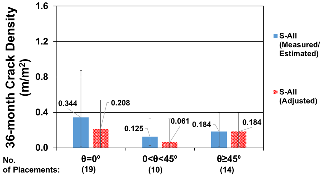
Figure E.7: Average measured/estimated and adjusted 36-month crack densities for all bridge decks supported by steel girders without fibers and different skew
