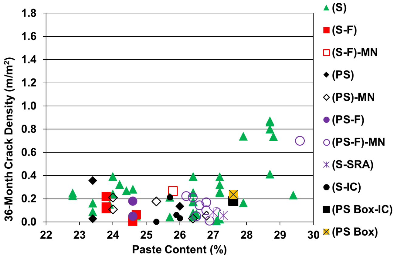
Figure 6.1: Paste content versus 36-month crack density for decks with good construction procedures
