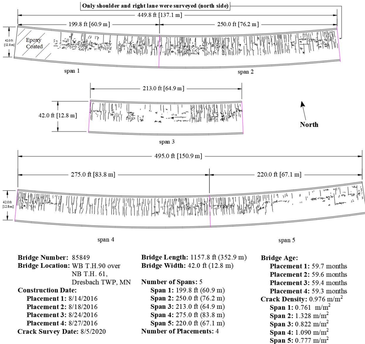
Figure 3.23: Crack survey of bridge 85849
