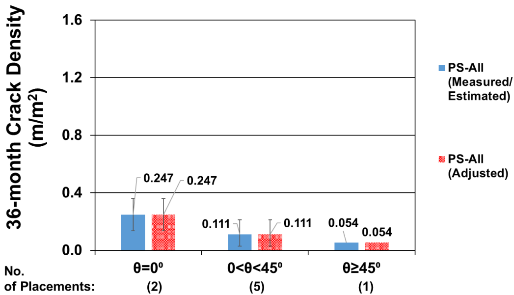
Figure E.5: Average measured/estimated and adjusted 36-month crack densities for all bridge decks supported by prestressed concrete girders without fibers and different skew
