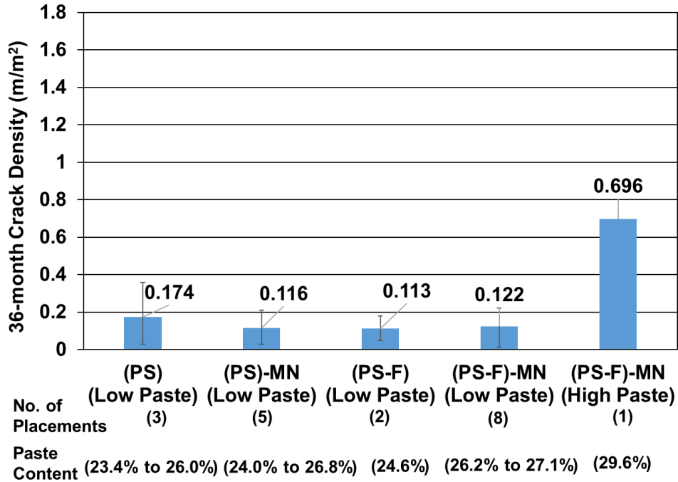
Figure 6.3: 36-month crack densities of decks supported by prestressed concrete girders with and without fibers
