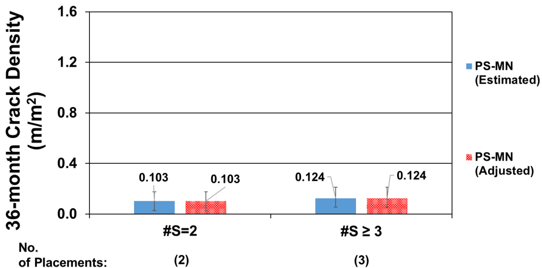
Figure E.16: Average measured/estimated and adjusted 36-month crack densities for Minnesota bridge decks supported by prestressed concrete girders without fibers and different numbers of span
