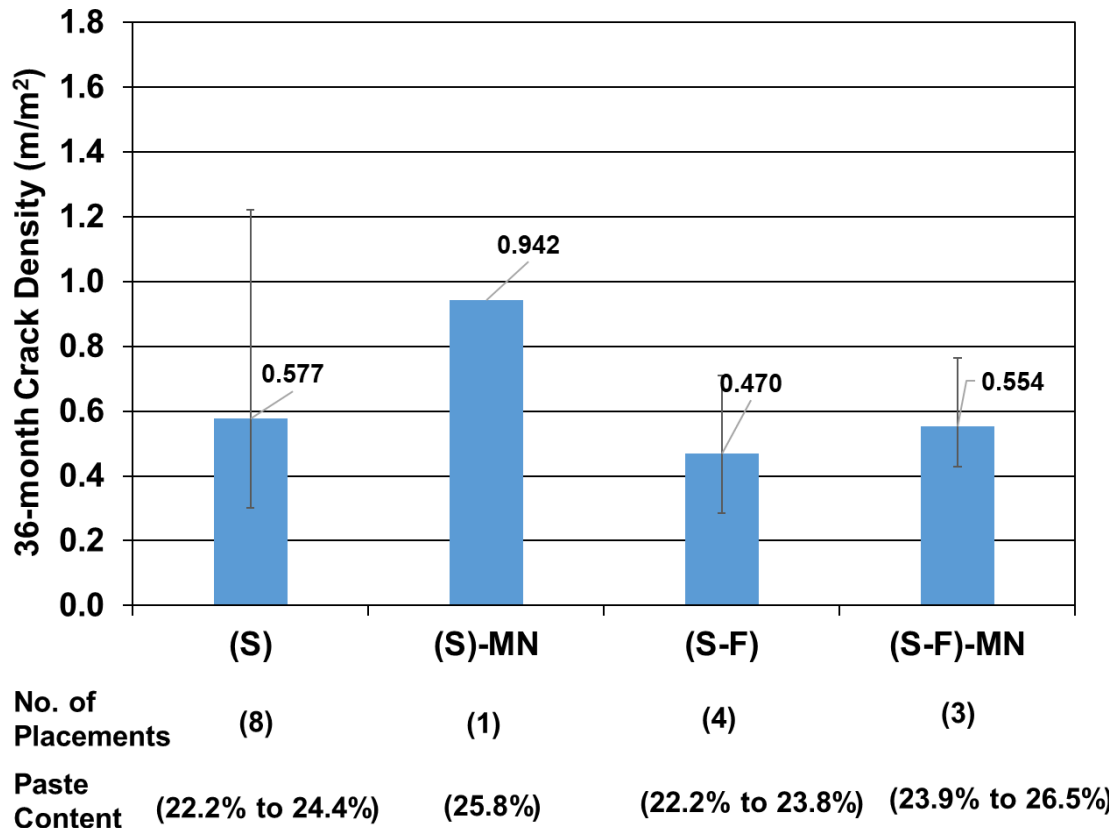
Figure 6.4: Comparing the 36-month crack densities of decks with construction issues
