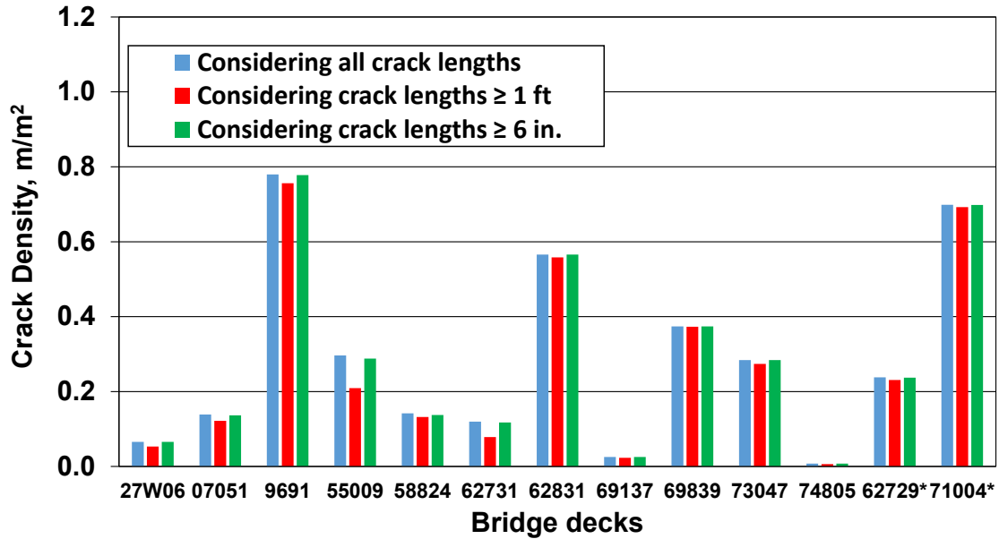
Figure 3.24: Comparison of crack densities, total, cracks with lengths \geq 1 ft (305 mm), and cracks with lengths \geq 6 in. (150 mm), for decks containing fibers
