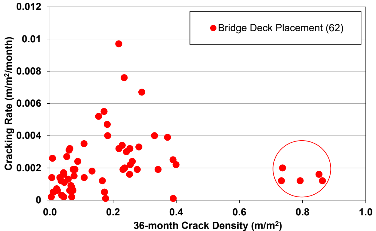
Figure C.2: Cracking rate versus 36-month crack density of 62 deck placements
