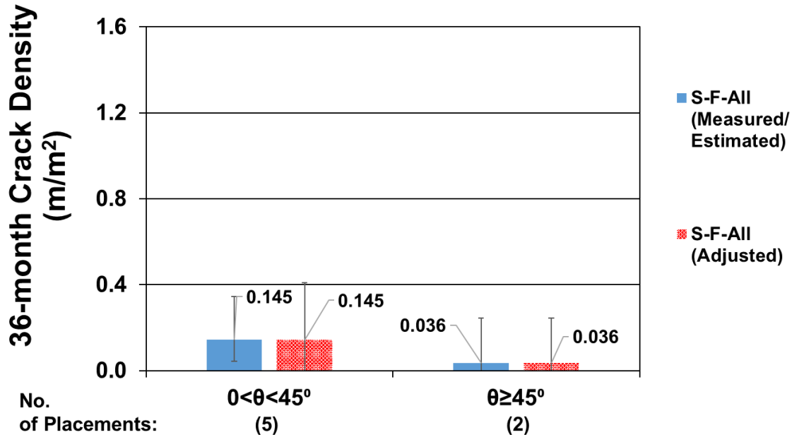
Figure E.6: Average measured/estimated and adjusted 36-month crack densities for all bridge decks supported by steel girders with fibers and different skew
