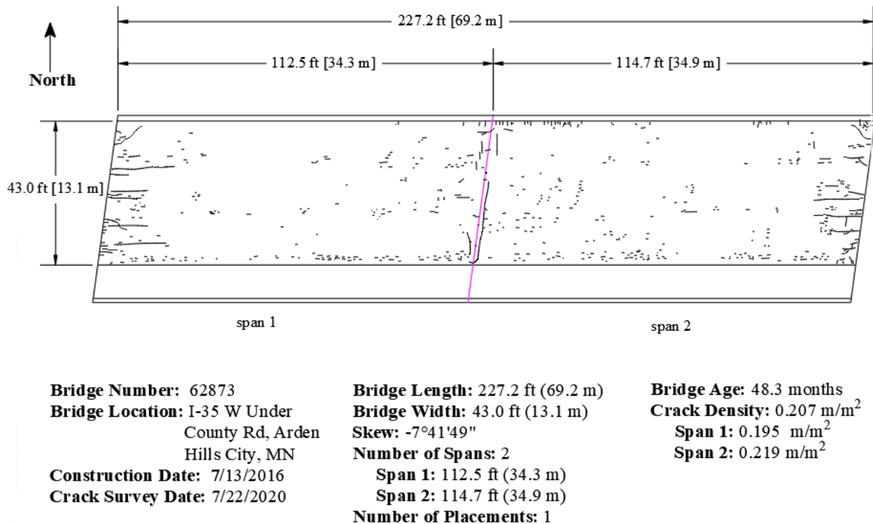
Figure 3.15: Crack survey of bridge 62873
