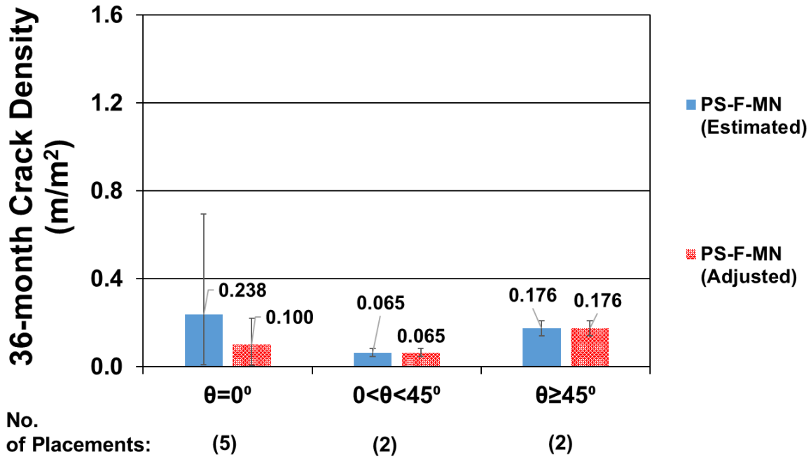
Figure E.1: Average measured/estimated and adjusted 36-month crack densities for Minnesota bridge decks supported by prestressed concrete girders with fibers and different skew
