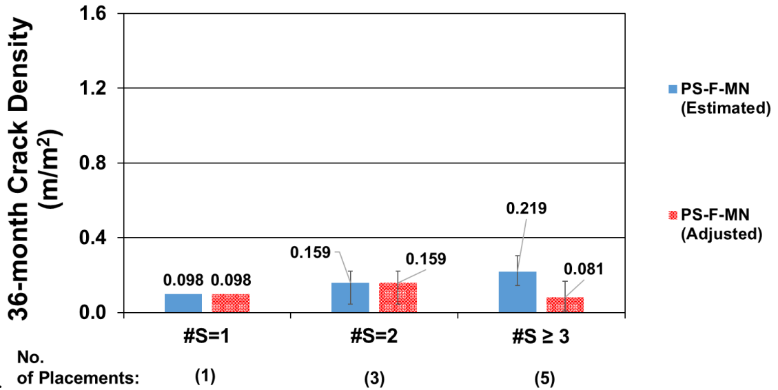
Figure E.15: Average measured/estimated and adjusted 36-month crack densities for Minnesota bridge decks supported by prestressed concrete girders with fibers and different numbers of span
