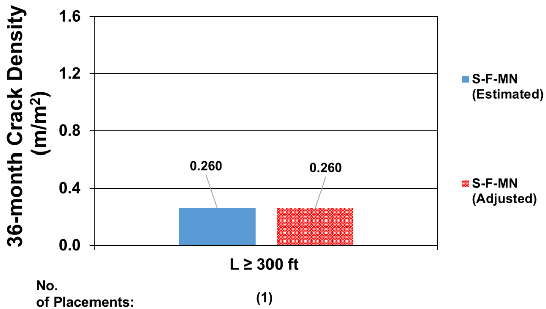
Figure E.10: Average measured/estimated and adjusted 36-month crack densities for a single Minnesota bridge deck supported by steel girders with fibers and a deck length greater than or equal to 300 ft ( L = 301.2 ft)
