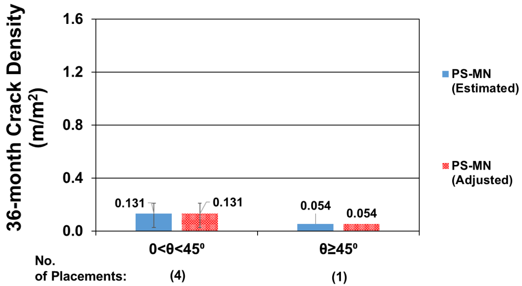
Figure E.2: Average measured/estimated and adjusted 36-month crack densities for Minnesota bridge decks supported by prestressed concrete girders without fibers and different skew
