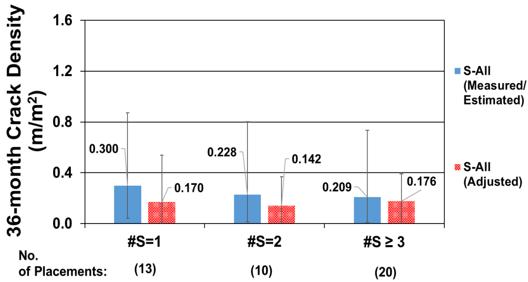
Figure E.21: Average measured/estimated and adjusted 36-month crack densities for all bridge decks supported by steel girders without fibers and different numbers of span
