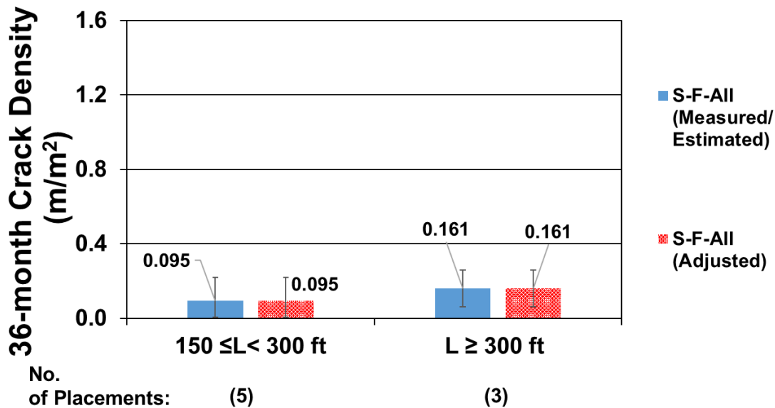
Figure E.13: Average measured/estimated and adjusted 36-month crack densities for all bridge decks supported by steel girders with fibers and different total deck length
