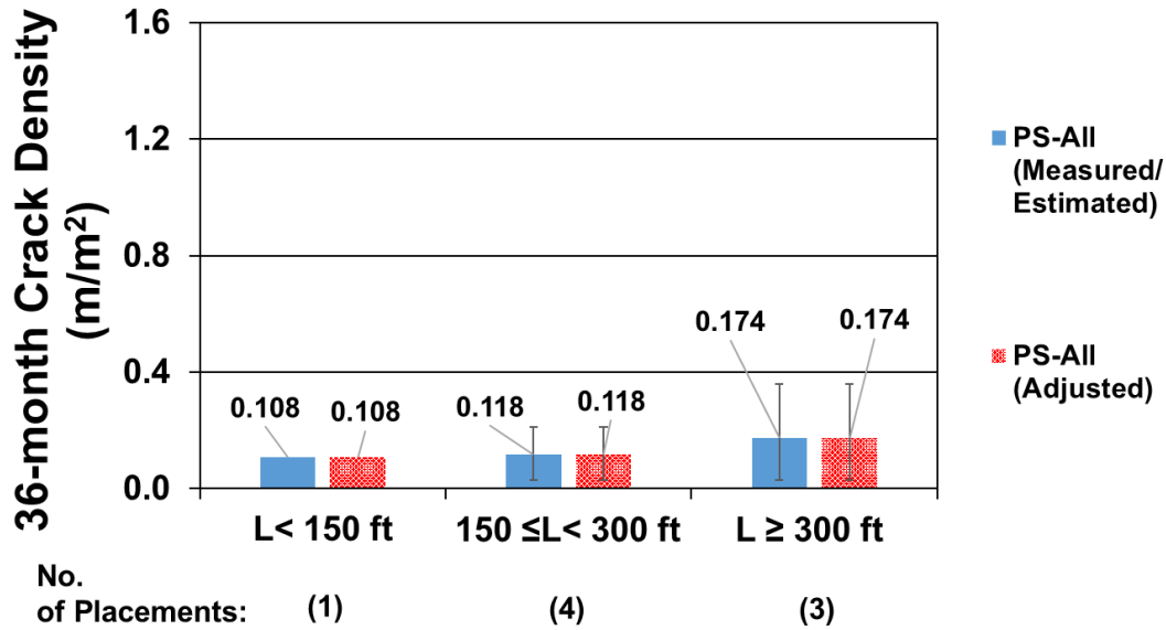
Figure E.12: Average measured/estimated and adjusted 36-month crack densities for all bridge decks supported by prestressed concrete girders without fibers and different total deck length
