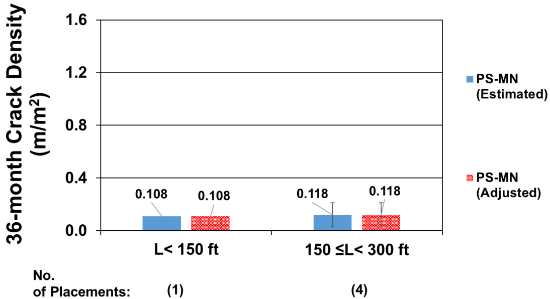
Figure E.9: Average measured/estimated and adjusted 36-month crack densities for Minnesota bridge decks supported by prestressed concrete girders without fibers and different total deck length
