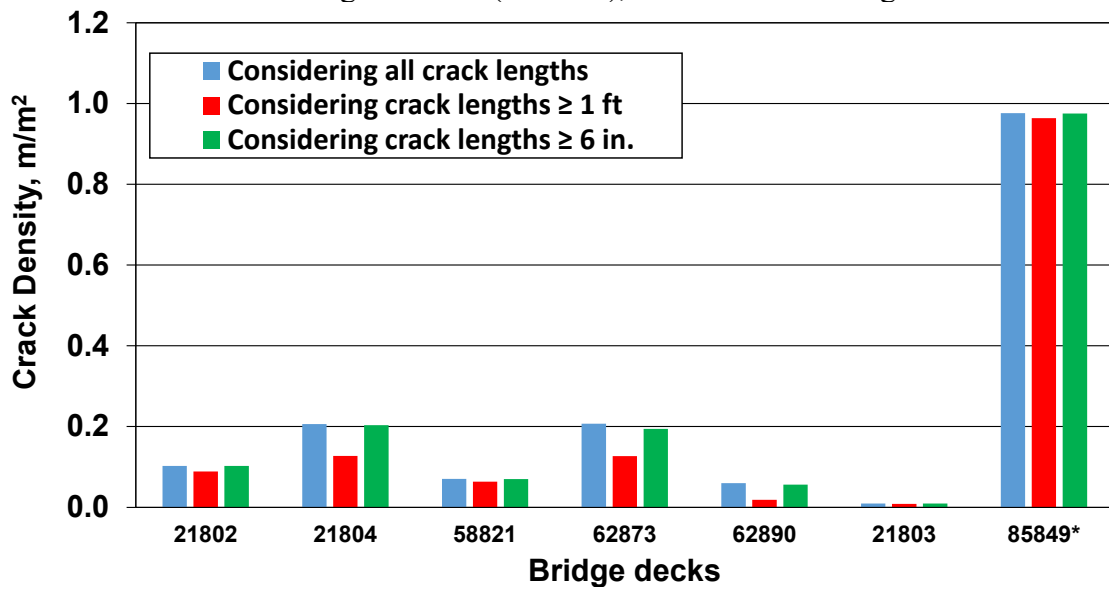
Figure 3.25: Comparison of crack densities, total, cracks with lengths \geq 1 ft (305 mm), and cracks with lengths \geq 6 in. (150 mm), for decks not containing fibers
