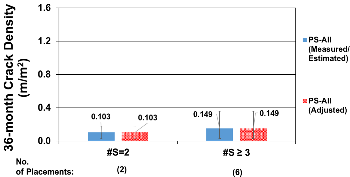
Figure E.19: Average measured/estimated and adjusted 36-month crack densities for all bridge decks supported by prestressed concrete girders without fibers and different numbers of span
