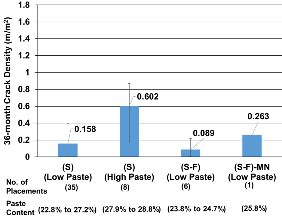
Figure 6.2: 36-month crack densities of decks supported by steel girders with and without fibers
