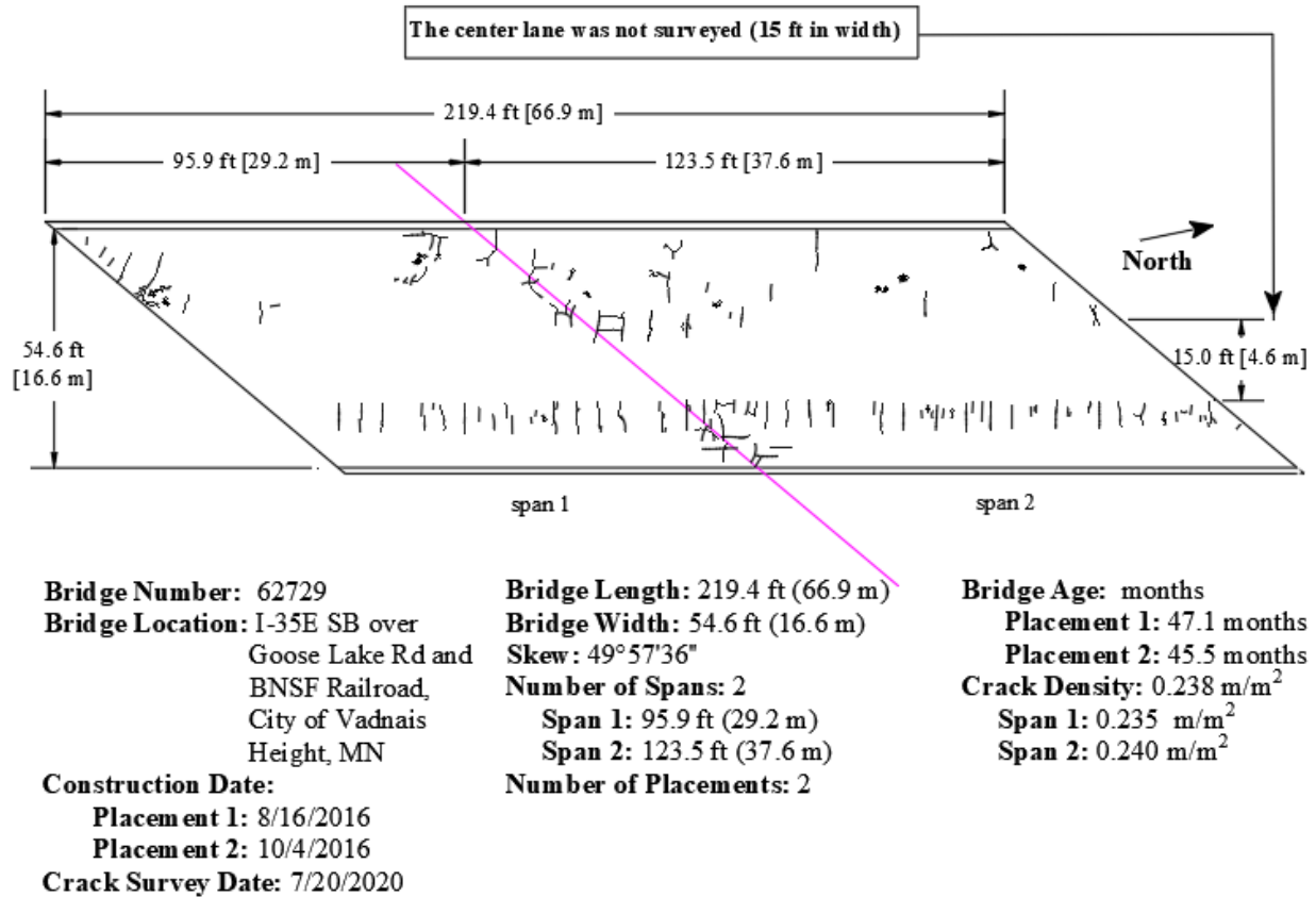
Figure 3.11: Crack survey of bridge 62729
