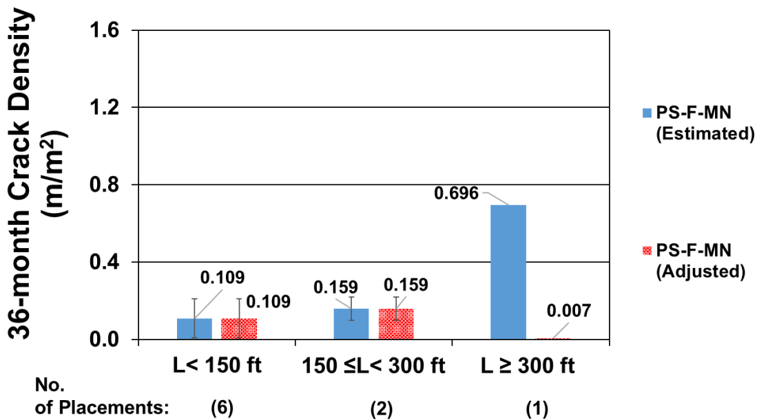
Figure E.8: Average measured/estimated and adjusted 36-month crack densities for Minnesota bridge decks supported by prestressed concrete girders with fibers and different total deck length
