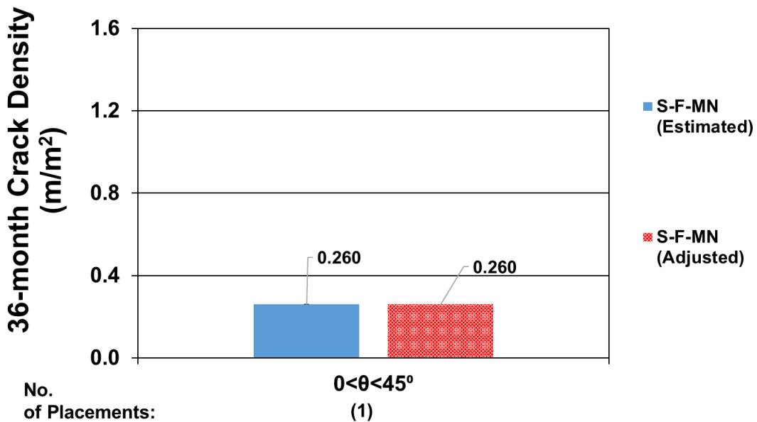
Figure E.3: Average measured/estimated and adjusted 36-month crack densities for a single Minnesota bridge deck supported by steel girders with fibers and a skew less than 45° ( \theta = 14^\circ )
