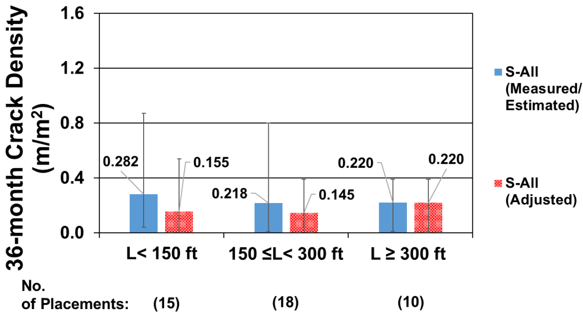
Figure E.14: Average measured/estimated and adjusted 36-month crack densities for all bridge decks supported by steel girders without fibers and different total length
