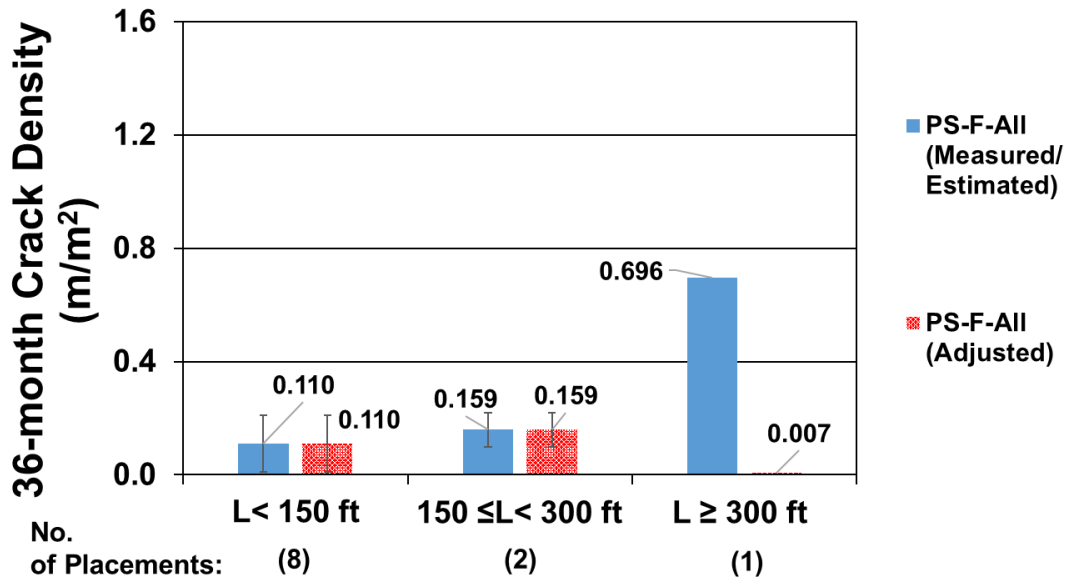
Figure E.11: Average measured/estimated and adjusted 36-month crack densities for all bridge decks supported by prestressed concrete girders with fibers and different total deck length
