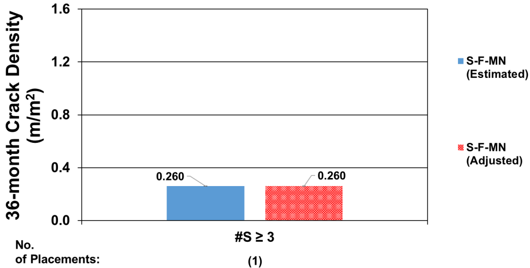
Figure E.17: Average measured/estimated and adjusted 36-month crack densities for a single Minnesota bridge deck supported by steel girders with fibers and four spans ( \#S \geq 3 )
