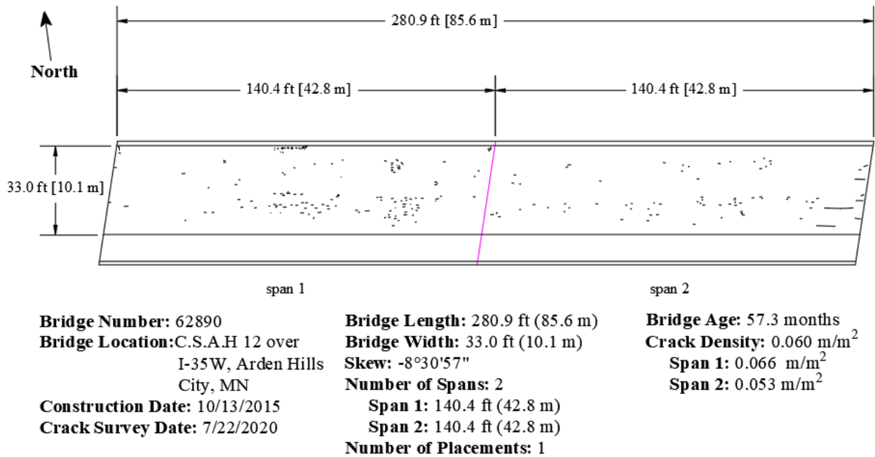
Figure 3.16: Crack survey of bridge 62890
