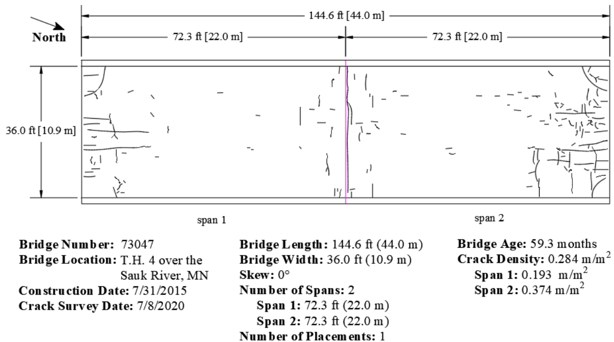
Figure 3.20: Crack survey of bridge 73047
