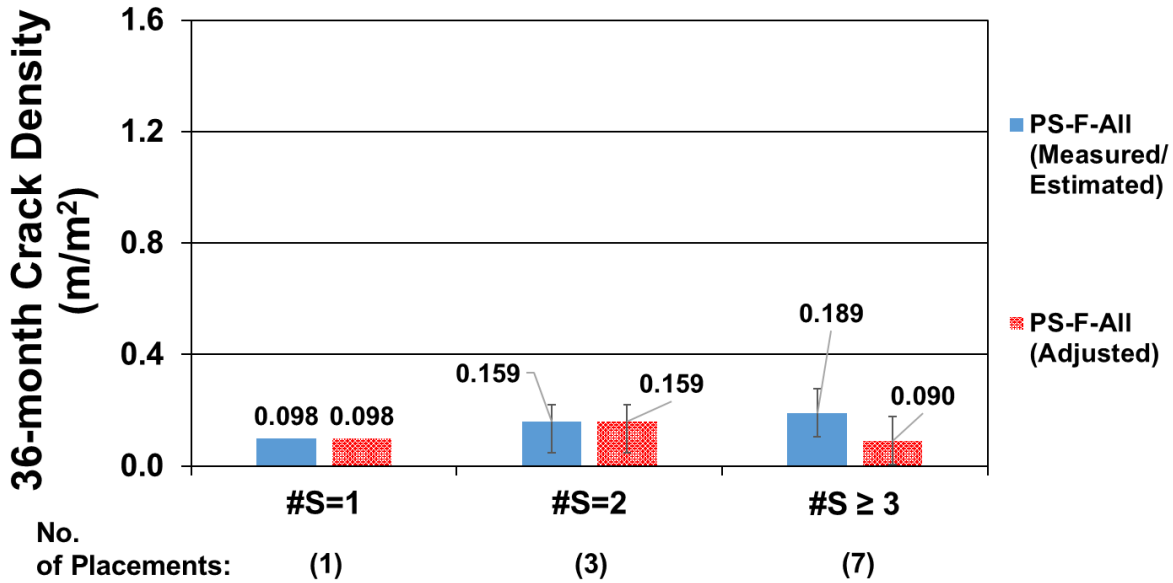
Figure E.18: Average measured/estimated and adjusted 36-month crack densities for all bridge decks supported by prestressed concrete girders with fibers and different numbers of span
