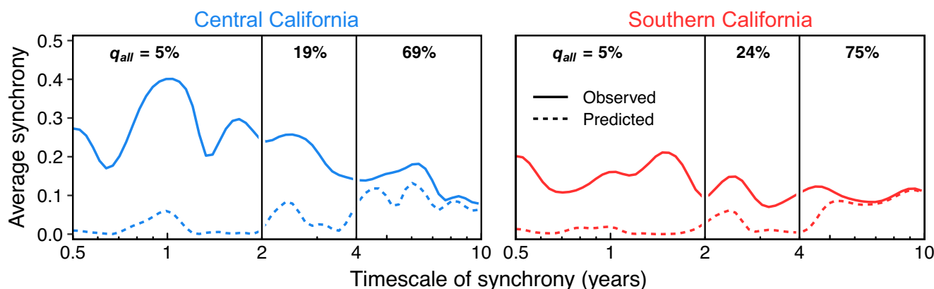
FIGURE 5 Synchrony of giant kelp canopy biomass is partly explained by fluctuations in the North Pacific Gyre Oscillation (NPGO), an oceanographic climate index that corresponds with large-scale strengthening of wind-driven upwelling. Lines and axes as in Figure 3. Numbers at the top of each timescale band show the average percentage of synchrony explained by NPGO wavelet models within a given region and timescale band ( q_{all} ; analogous to black bars for total synchrony explained in Figure 4)
