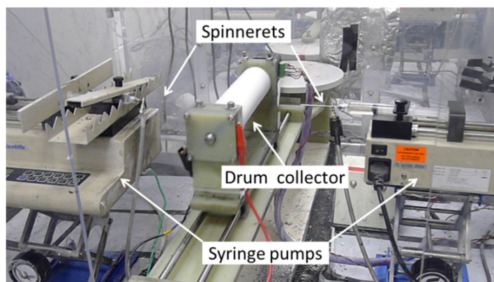
Figure 1. Schematic of the dual fiber electrospinning setup used in the present study.
