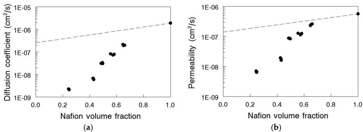
Figure 6. (a) Diffusion coefficient of bromine species ( \text{Br}_2 and \text{Br}_3^- ) in Nafion nanofiber composite membranes of different Nafion volume fractions at 25^\circ\text{C} . Diffusion coefficient of Nafion® 115 was 1.45 \times 10^{-6} \text{ cm}^2/\text{s} ; (b) Steady-state permeability of bromine species ( \text{Br}_2 and \text{Br}_3^- ) for the nanofiber composite membranes as a function of Nafion volume fractions at 25^\circ\text{C} . Steady-state permeability of Nafion® 115 was 4.26 \times 10^{-6} \text{ cm}^2/\text{s} .
