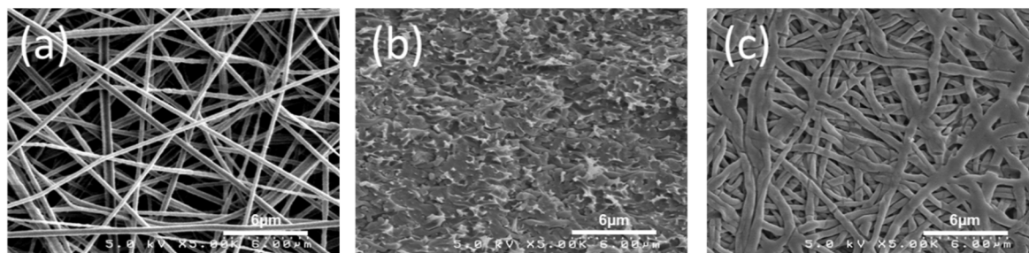
Figure 3. SEM images of (a) an electrospun Nafion/PPSU dual nanofiber mat; (b) freeze-fractured cross section of 57 vol% N(fibers)/PPSU; and (c) surface of the Nafion fiber structure after extraction of all PPSU with liquid chloroform. Magnification 5,000X.
