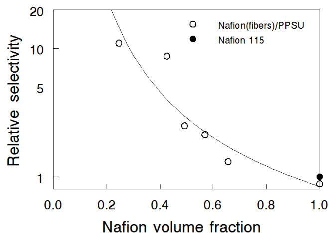
Figure 7. Relative, with respect to Nafion 115, selectivity of the nanofiber composite membranes as a function of Nafion volume fractions at 25 °C. (○) N(fibers)/PPSU; (●) Nafion ® 115.
