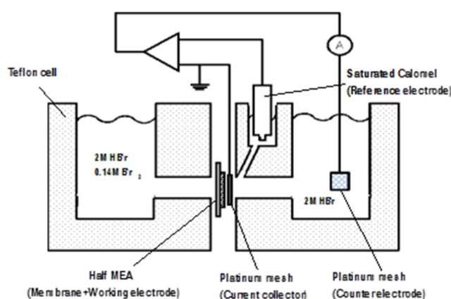
Figure 2. Schematic diagram of the two compartment apparatus for determining membrane diffusion coefficients.
