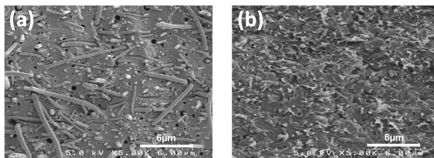
Figure 9. SEM micrographs of the cross-sections of two 57 vol% Nafion/PPSU membranes with complementary morphologies: (a) N/PPSU(fibers)-PPSU nanofibers embedded in a Nafion matrix; and (b) N(fibers)/PPSU-Nafion nanofibers embedded in a PPSU matrix. Magnification is 5,000X.
