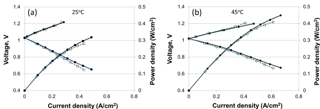
Figure 10. H 2 /Br 2 regenerative fuel cell performance at 25 °C (a) and 45 °C (b) with a 55 vol% N (fibers)/PPSU nanofiber composite membrane, 65 μm in thickness (●); and Nafion 115 membrane, 140 μm in thickness (○). Plots show both charging and discharging curves [34]. Adapted with permission from J. Electrochem. Soc. , 162, F919 (2015). Copyright 2015, The Electrochemical Society.
