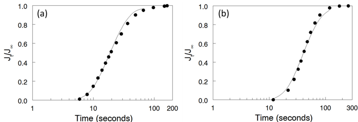
Figure 5. Fit of experimental data to the transient breakthrough model for: (a) Nafion® 115; and (b) 57 vol% N (fibers)/PPSU nanofiber composite membrane. Figure 5a adapted with permission from ECS Transactions, 50 (2) 1217 (2012). Copyright 2012, The Electrochemical Society.
