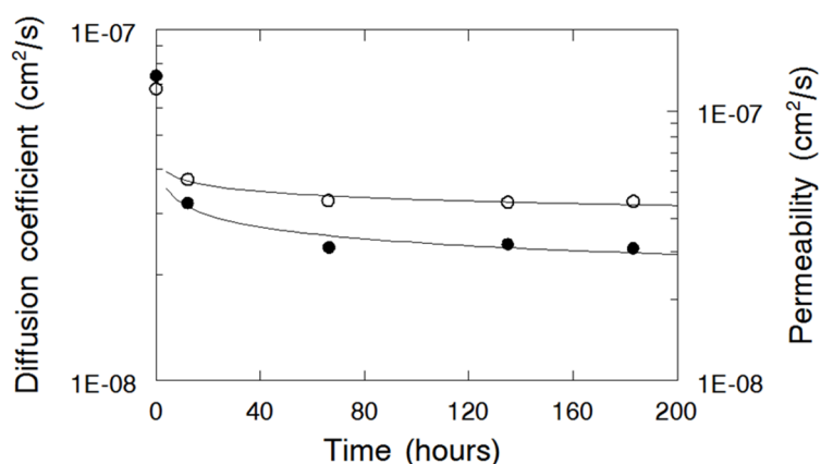
Figure 8. Diffusion coefficient (●); and steady-state permeability (○) of \text{Br}_2/\text{Br}_3^- in N(fibers)/PPSU nanofiber composite membrane as a function of soak time in a solution of 0.14 M \text{Br}_2 in 2 M HBr at 25 °C.
