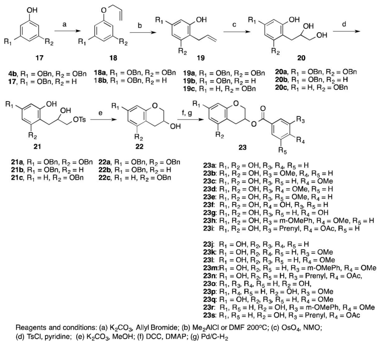
Scheme 4. Synthesis of esters of 3,5-dihydroxychroman-3-ol.
