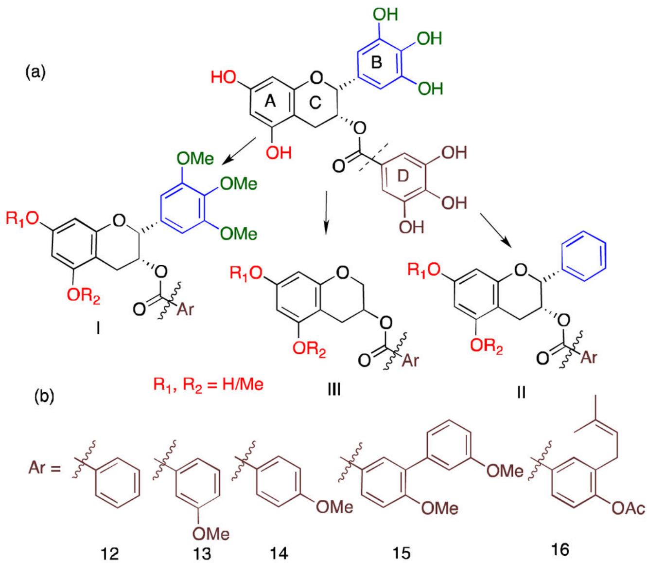
Scheme 2.
