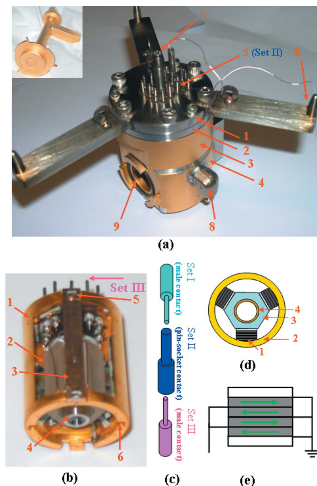
FIG. 3. (Color online) High pressure reactor and STM body. (a) A view of the whole reactor: (1) cell lid, (2) cell neck, (3) middle stage, (4) bottom stage, (5) pin-socket contacts for wiring of STM body at the interface of high vacuum and high pressure environment, (6) a pin on the lever of the cell lid for mounting, (7) Swagelok fitting welded on the tube of the cell lid for gas introduction, (8) Swagelok fitting welded on the button stage of reactor for sample and tip transfer. (b) Side view of the STM body: (1) wall of STM body coated with a layer of gold, (2) hexagonal sapphire, (3) CuBe spring plates, (4) receiver of tip holder, (5) screw to adjust the pressure applied to hexagonal sapphire, and (6) hole to assemble sample stage to STM body. (c) Scheme of pin-socket alignment for wiring. Set III is the contacts glued to the holes on top of STM body; set II is the contacts glued to the holes on top of cell lid of the reactor; set I is the contacts glued to wires from docking scaffold. (d) Scheme showing the assembly of three packs of shear piezoelectric plates between the hexagonal sapphire and the wall of the STM body and the assembly of the scanning tube: (1) a set of piezoelectric plates, (2) wall of STM body, (3) hexagonal sapphire, and (4) scanning tube. (e) Scheme showing how the four shear piezoelectric plates of one set work for coarse approach. Two alumina plates are glued to the first and fourth shear piezoelectric plates for thermal isolation and electrical insulation.
