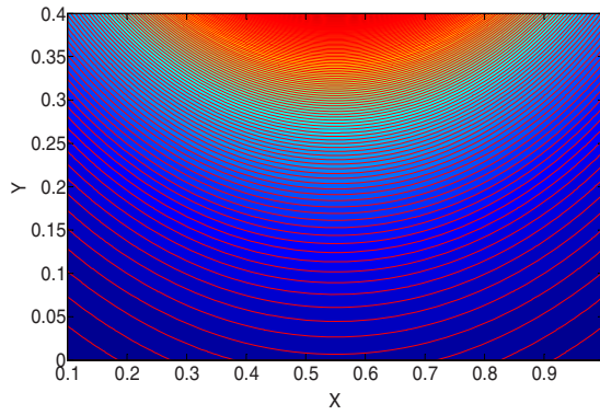
FIG. 1. (Color online) Electric field intensity distribution generated by the charged globe.
