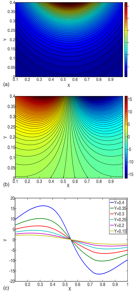
FIG. 2. (Color online) [(a)–(c)] Components of the force generated by the gradient dc electric field in the vertical y direction, in the horizontal x direction, and the x direction field at different y values, respectively.
