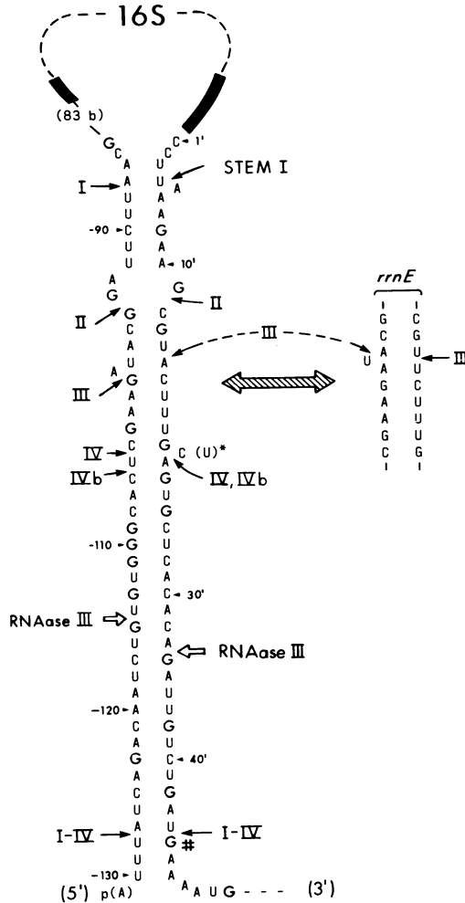
FIGURE 5. Sequence and secondary structure of stems isolated from pl6b rRNA. RNase-resistant oligonucleotides (from Table 3) are arranged according to the DNA sequences of the rrnD and X operons (8); the homologous sequence in rrnE (right) is from Ref. 18. Arrows indicate the extent of the isolated stems I through IVb (Figure 3): they are placed as described in the text. To facilitate reference to the text and to Table 3, the terminal G of each T1 oligonucleotide is in bold face, and nucleotide positions prior to the 5' end of m16 (negative numbers) and past the 3' end (primed numbers) are numbered. The solid bars indicate the termini of mature 16S rRNA. Location of the RNase III cleavage site in 30S rRNA, between positions -114 and -115 and 33'/34', is from Refs. 2 and 23. * , C is replaced by U in rrnB (C. Squires and C. Squires, personal communication);# , the sequence of rrnB and E begins to diverge from that shown here.
