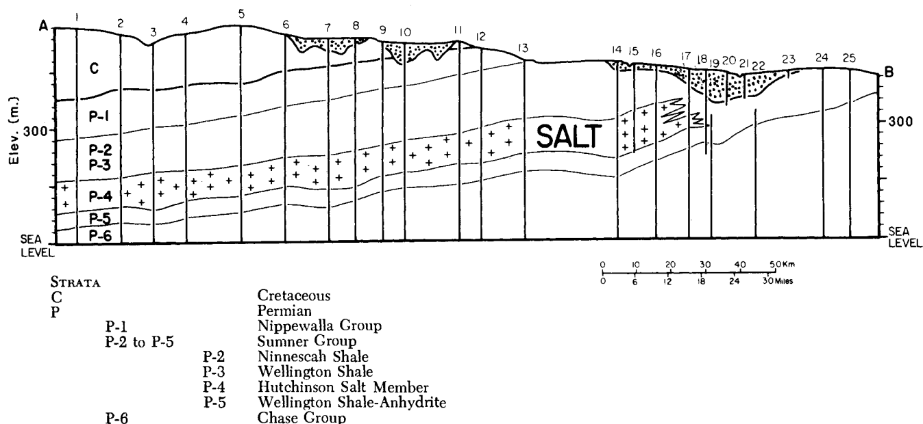
FIG. 2. Cross-section A-B of Figure 1. Rock unit names below the figure correspond to labels on the figure. Locations of wells drilled for oil, gas, and water are depicted by numbers along the top of the cross-section. Modified from Walters (1977) where the well locations are listed and discussed.
