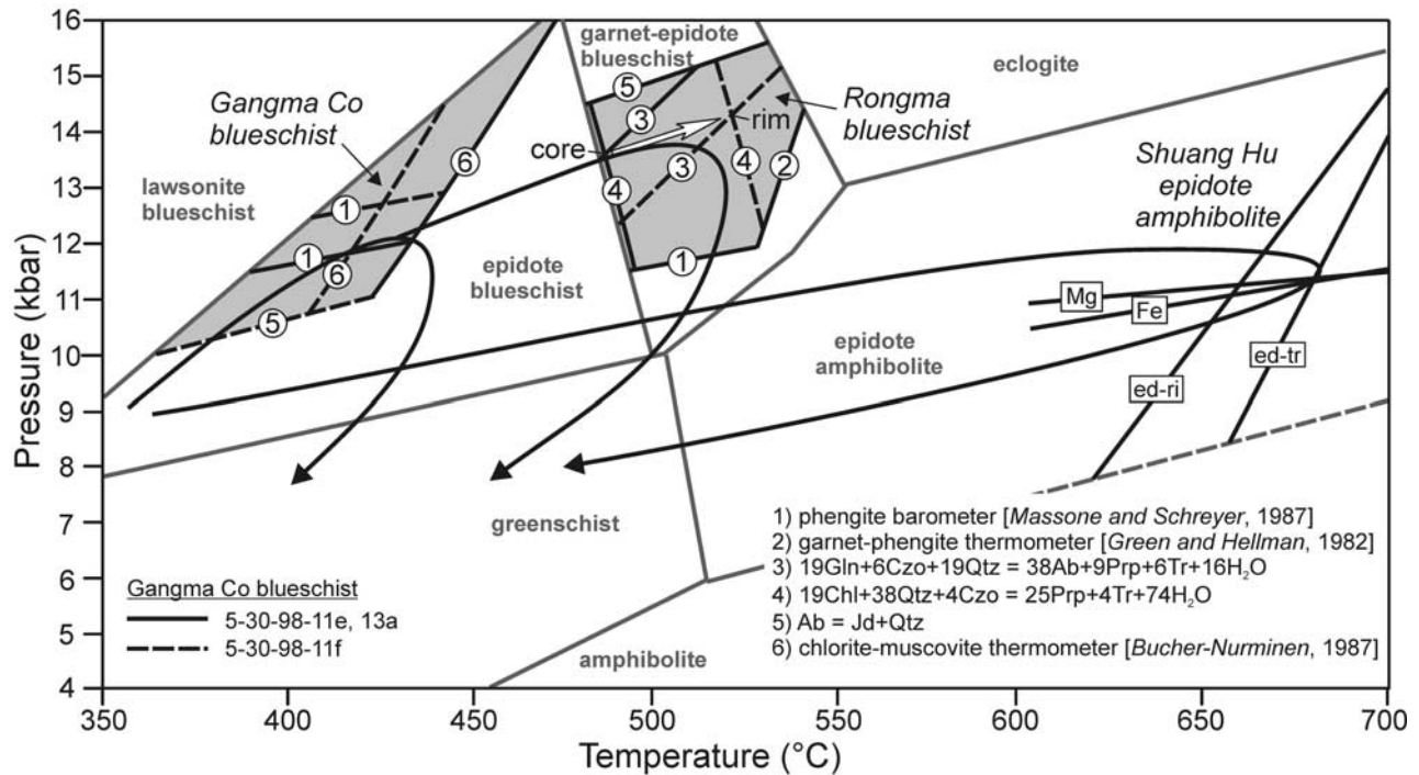
Figure 7. Summary of thermobarometric results for Gangma Co blueschist, Rongma blueschist, and Shuang Hu epidote amphibolite. Schematic P-T paths are based on thermobarometric results coupled with observed mineral parageneses and textural relationships. The dark gray metamorphic facies boundaries are from Evans [1990], calculated for a theoretical metabasite with mineral compositions similar to those determined for Gangma Co and Rongma blueschists. The dashed boundary between epidote-amphibolite and amphibolite facies is extrapolated from that of Evans [1990] at T \leq 600^\circ\text{C} . Clinopyroxene from Gangma Co sample 5-30-98-11f was used to calculate the equilibrium: \text{Ab} = \text{Jd} + \text{Qtz} ; clinopyroxene in samples 5-30-98-11e and 5-30-98-13a were not used because they were found to be complexly zoned with relict igneous cores and metamorphic rims. Phengite barometry and chlorite-muscovite thermometry provide minimum P and maximum T estimates, respectively, because K-feldspar is absent and water is assumed to have an activity of 1.0. Phengite from Rongma blueschist yield Mg numbers [ 100 \times \text{Mg}/(\text{Mg} + \text{Fe}) ] of \sim 62 , and the equation of Green and Hellman [1982] interpolated for basaltic systems with Mg number of 67 was used for garnet-phengite thermometry. The magnesium (Mg) and iron (Fe), and edenite-richterite (ed-ri) and edenite-tremolite (ed-tr), end-member equilibria were used for garnet-hornblende-plagioclase barometry [ Kohn and Spear , 1990] and hornblende-plagioclase thermometry [ Holland and Blundy , 1994] of Shuang Hu epidote amphibolite, respectively.
