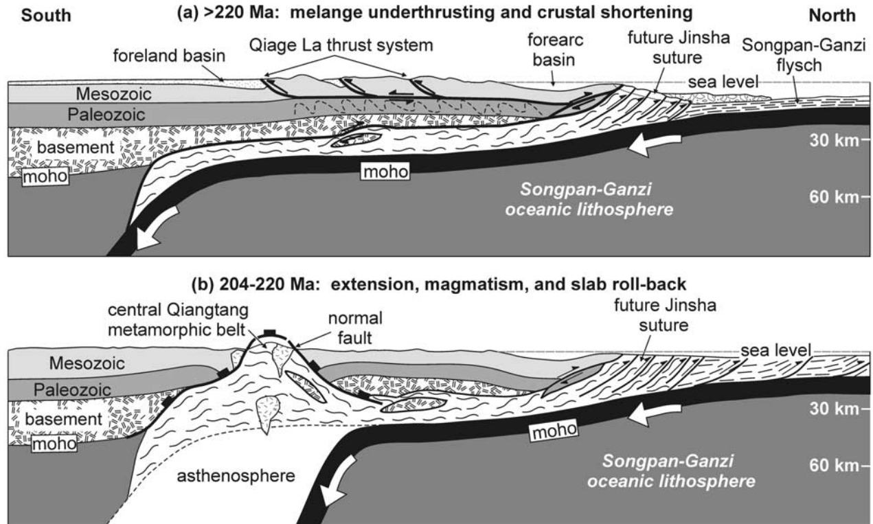
Figure 12. Two-stage model for the early Mesozoic tectonic evolution of central Qiangtang metamorphic rocks that elaborates on the melange underthrusting model of Kapp et al. [2000] and Kapp [2001]. (a) Melange underthrust southward beneath the Qiangtang continental margin during Triassic low-angle oceanic subduction along the Jinsha suture. The Qiage La thrust system accommodated upper crustal shortening during this time. (b) Exhumation of underthrust melange to upper crustal levels by Late Triassic–Early Jurassic normal faulting, coeval with ongoing subduction. Extension and magmatism may have been initiated by rollback of the subducting oceanic lithosphere. This model predicts that the northern Qiangtang continental mantle was tectonically removed during early Mesozoic time and that the present-day deeper crust of the northern Qiangtang terrane includes large volumes of underthrust early Mesozoic melange.
