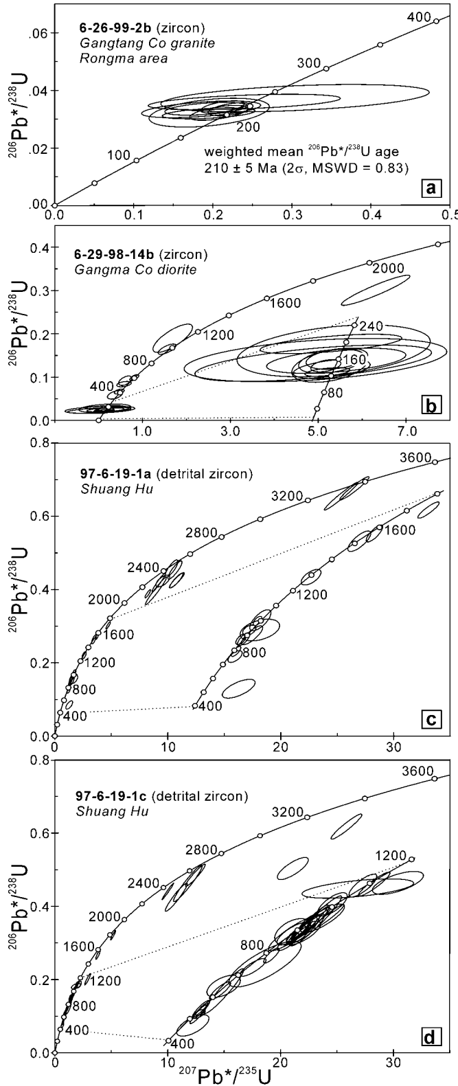
Figure 9. Concordia plots of U-Pb ion microprobe single-spot analyses (error ellipses are 2\sigma ) of zircons from the (a) Gangtang Co granite, (b) Gangma Co diorite, and (c–d) metasediments in the footwall of the Falong detachment, Shuang Hu area.
