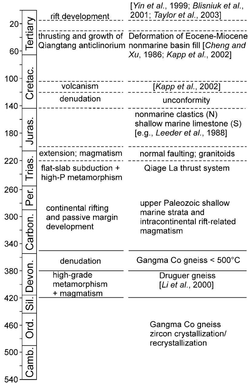
Figure 11. Summary of the Paleozoic–early Mesozoic tectonic evolution of the Qiangtang terrane.
