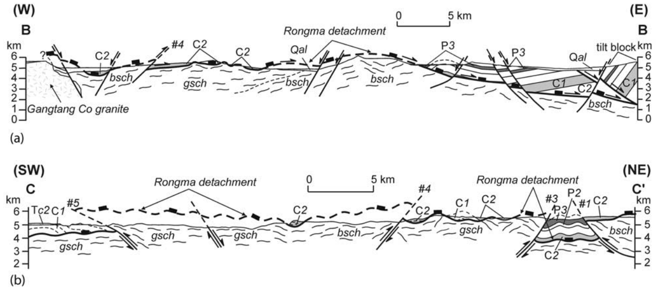
Figure 6. (a) East-west, B–B'; Early Mesozoic normal faults are bolder than younger faults and (b) northeast-southwest, C to C' cross sections of the Rongma area. See Foldout 2 for lines of section and unit abbreviations. Abbreviations are: gsch, greenschist-facies melange; bsch, blueschist-facies melange; C1, Carboniferous quartzite-bearing siliciclastic rocks; C2, Carboniferous limestone-bearing strata; P1, Permian turbiditic sandstone; P2, Permian limestone; P3, Permian mafic volcanic rocks and conglomerates; P4, Permian limestone and sandstone; Ts2, Tertiary nonmarine strata; N-Q, Neogene-Quaternary conglomerate; Qal, Quaternary alluvium.
