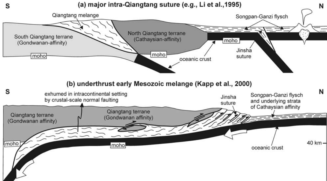
Figure 2. Competing hypotheses for the tectonic significance of the central Qiangtang metamorphic belt during early Mesozoic time.
