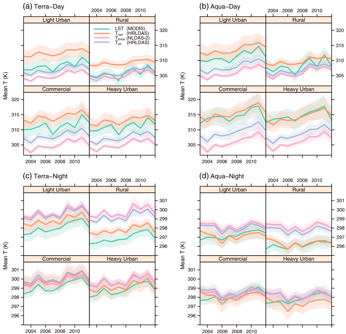
Figure 7. The 2003–2012 domain average, annual average JJA temperatures for four surface types for MODIS LST, HRLDAS T_{rad} , NLDAS-2 T_{force} , and HRLDAS T_{air} for Terra and Aqua (a, b) daytime and (c, d) nighttime passes. HRLDAS results are from experiment D2. The shaded areas indicate \pm 1 standard deviation from the 10 year average for each land cover type.
