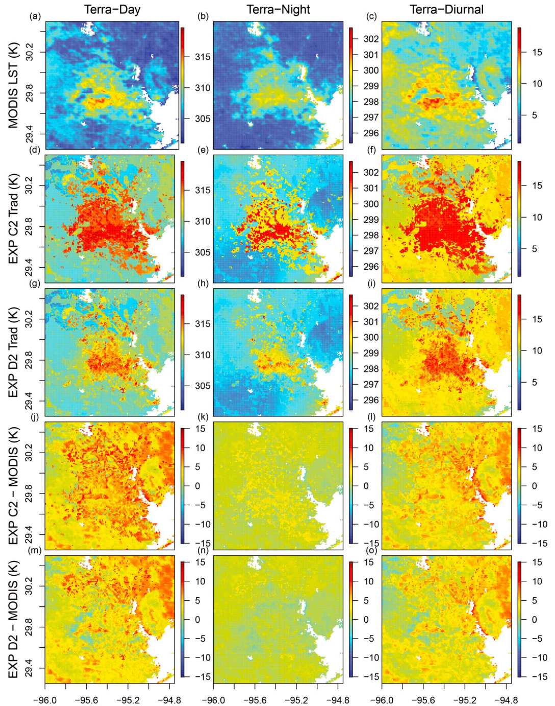
Figure 5. The 2003–2012 average JJA (row 1) MODIS LST (Terra) and (rows 2 and 3) HRLDAS T_{rad} for experiments C2 and D2, for (column 1) day, (column 2) night, and (column 3) difference of day and night (diurnal). (rows 4 and 5) The difference maps for HRLDAS minus MODIS for experiments C2 and D2 are shown.
