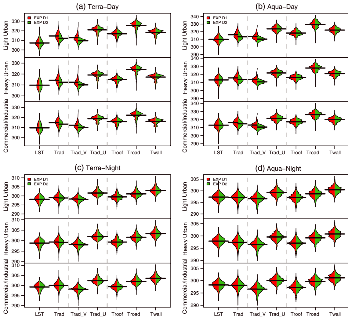
Figure 4. Comparison of the 2003–2012 JJA distributions of MODIS LST with the components of HRLDAS T_{rad} (K; left axis) for Terra and Aqua (a, b) daytime and (c, d) nighttime passes. Scenarios are grouped by experiment D1 (red) and D2 (green), as well as by (top) light-intensity, (middle) heavy-intensity, and (bottom) commercial/industrial-intensity land use types. The component temperatures for HRLDAS T_{rad} ( T_{rad\_v} , T_{rad\_u} , T_{roof} , T_{road} , and T_{wall} ) are described in the methods section. The black bars represent mean values.
