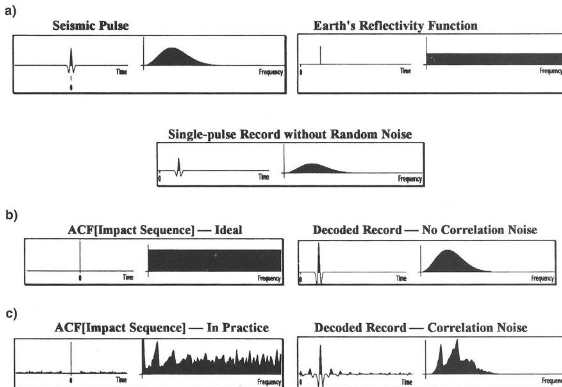
FIG. 2. The goal of a coded impact seismic technique is to amplify the seismic pulse on (a) the single-pulse record without distortion of its original shape. An ideal ACF (b) achieves this goal, whereas, in practice, the ACF from a coded impact seismic technique deviates from the ideal one and results in correlation noise on the decoded record.
