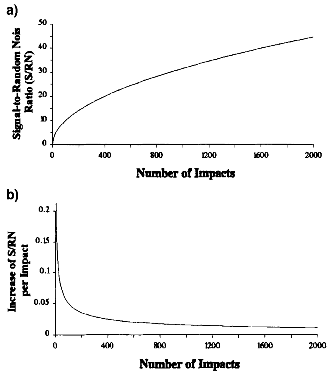
FIG. 3. (a) The square-root relationship between the signal-to-random noise ratio (S/RN) improvement and the total number of impacts ( N ) in a coded impact seismic technique. (b) Increment of S/RN with N per impact.
