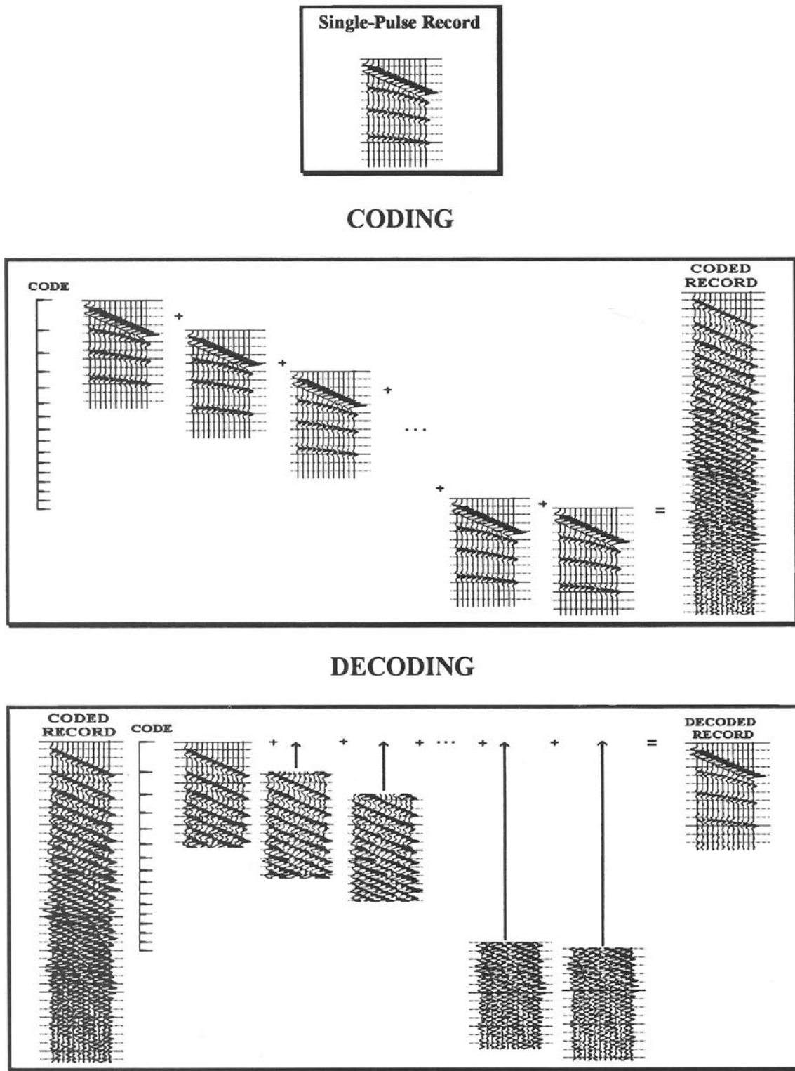
FIG. 4. Schematic of the coding and decoding process of SIST. The coding process is identical to assigning a single-pulse record into each impact instant (impact time break), and the coded record is formed from the superposition of all the assigned records. During the decoding process, a subrecord much shorter than the coded record is extracted from the coded record beginning at each impact time, shifted to the zero time, and then stacked with all other shifted subrecords to produce a decoded record.
