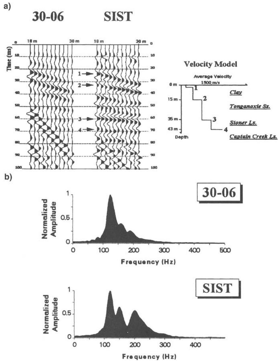
FIG. 13. (a) Processed (band-pass filtered and AGC applied) versions of the records shown in Figure 12a. Only the top 100 ms portions are displayed. Interpretation of the SIST record is shown on the right-hand side. (b) Average amplitude spectra for the 60 ms reflections on both records. Air-coupled wave echoes were carefully eliminated before the calculation of spectra.
