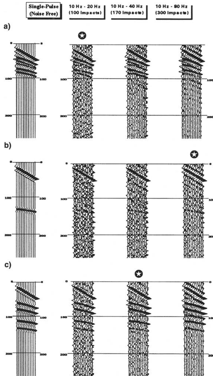
FIG. 9. Optimum ending impact rate is determined based upon relative significance of S/CN and S/RN in the interpretation. The preliminary determination depends upon the way the target reflections occur. Three cases where this can occur are illustrated as: (a) target reflections (5 reflections) occur in close to each other, (b) target reflection occurs in isolation, and (c) intermediate between (a) and case 2(b). Three different f_e 's are modeled and the possible optimum f_e is indicated by ★ in each case. The same degree of random noise had been included during the modeling.
