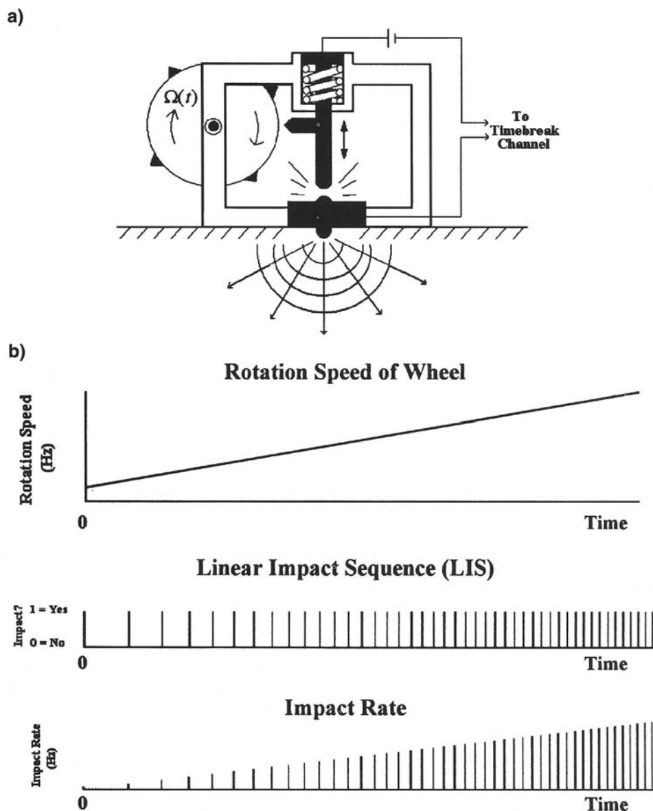
FIG. 5. (a) Diagram of a simple device that can produce a temporally varying rate of impacts. A time break circuit is closed at each impact, and one time break pulse is generated to be recorded on a separate channel. (b) If the rotation speed of the wheel changes linearly with time, so does the impact rate. The impact sequence created this way is called linear impact sequence (LIS).
