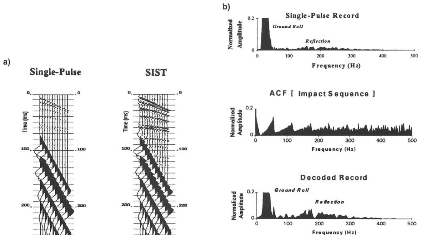
FIG. 7. SIST modeling to illustrate low-cut filter effect of LIS on decoded record. (a) A single-pulse record and a decoded SIST record. (b) Amplitude spectra of the single-pulse record, auto-correlation of the LIS, and the decoded record. Ground-roll amplitudes have been clipped for display purpose.
