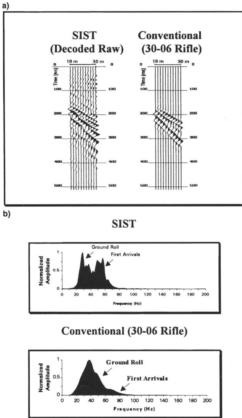
FIG. 12. (a) Decoded SIST record whose coded version is displayed in Figure 10b. Accept for decoding, no other processing has been applied. A conventional single-pulse field record obtained by using 30-06 rifle (Miller et al., 1992) as a source is displayed also for comparison purposes. (b) Average amplitude spectra for each type of record.
