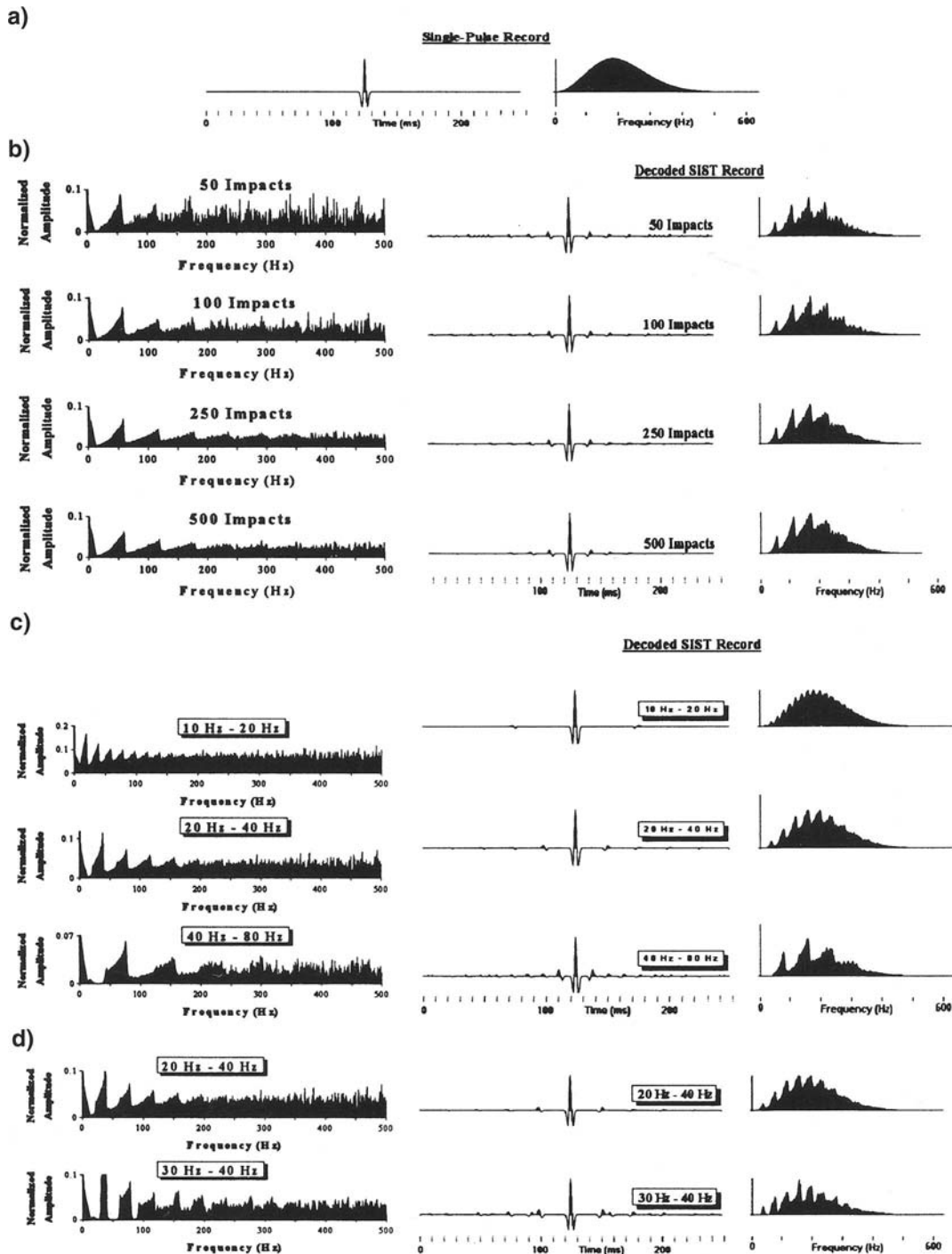
FIG. 8. Effects of changing (b) the total number of impacts ( N ), (c) starting ( f_s ) and ending ( f_e ) impact rates, and (d) bandwidth of impact rates ( dF ) on correlation noise. Inputs to the modeling included a (a) 180 Hz Ricker wavelet and different LIS's. Power spectra of LIS's (left), decoded wavelets (center), and the amplitude spectra of the decoded wavelets (right) are displayed in the test of each parameter.
