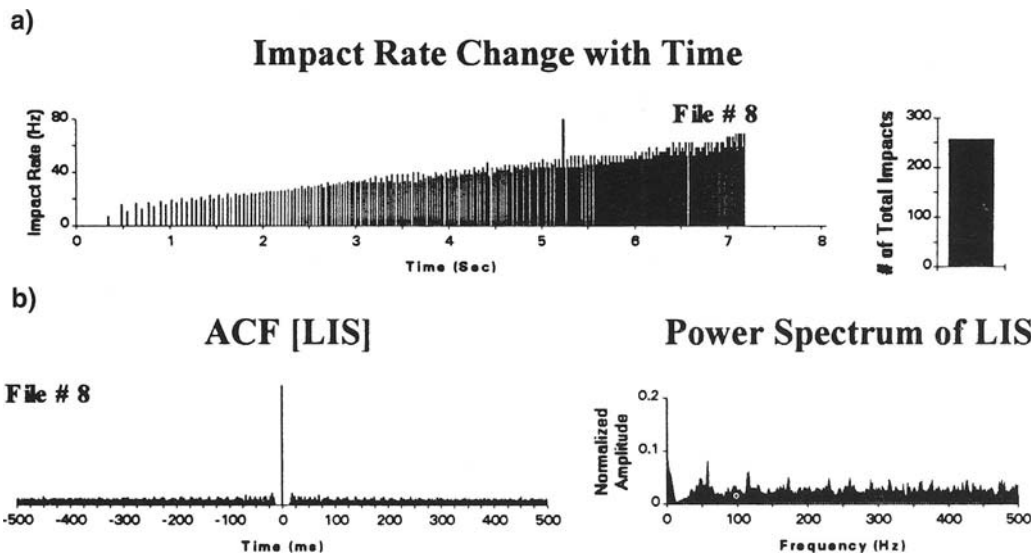
FIG. 11. (a) Plot of impact rate change with time for the SIST record shown in Figure 10a. There are about 250 impacts delivered. Time and amplitude of each spike in the plot represent the impact instant and the impact rate, respectively. (b) ACF and power spectrum of the impact sequence.
