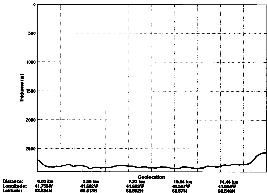
Figure 3c. Ice thickness obtained from the radar data collected over the central part of the ice sheet. (The radar data have been averaged over a distance covered by aircraft in \sim 0.139 s ( \sim 18 m).)
