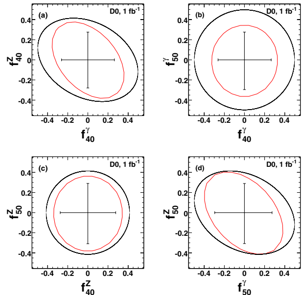
FIG. 1 (color online). Limits on anomalous couplings for \Lambda = 1.2 TeV: (a) f_{40}^\gamma vs f_{40}^Z , (b) f_{40}^\gamma vs f_{50}^\gamma , (c) f_{40}^Z vs f_{50}^Z , and (d) f_{50}^\gamma vs f_{50}^Z , assuming in each case that the other two couplings are zero. The inner and outer curves are the 95% C.L. two-degree of freedom exclusion contour and the constraint from the unitarity condition, respectively. The inner cross hairs are the 95% C.L. one-degree of freedom exclusion limits.
