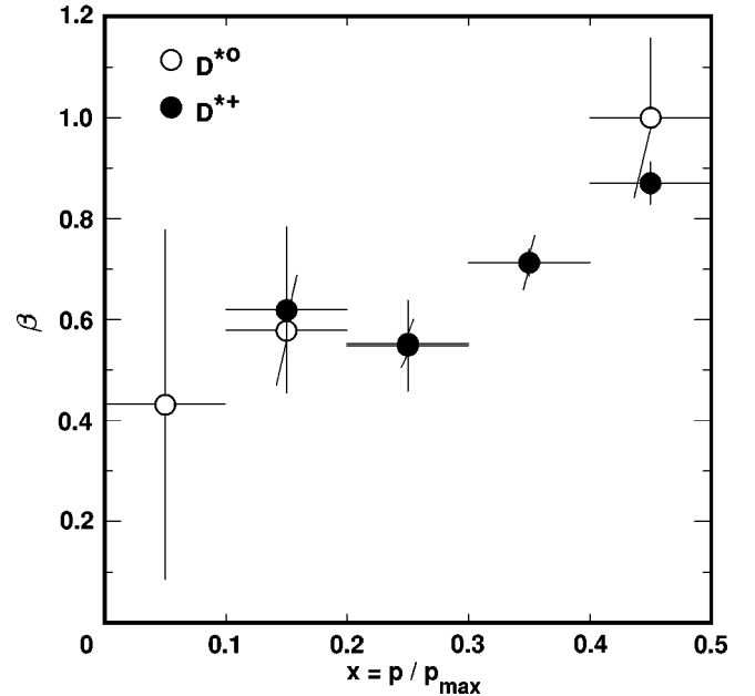
FIG. 36. \beta(D^*) vs x = p/p_{\max} ( p_{\max} = 4.950 GeV/c).
