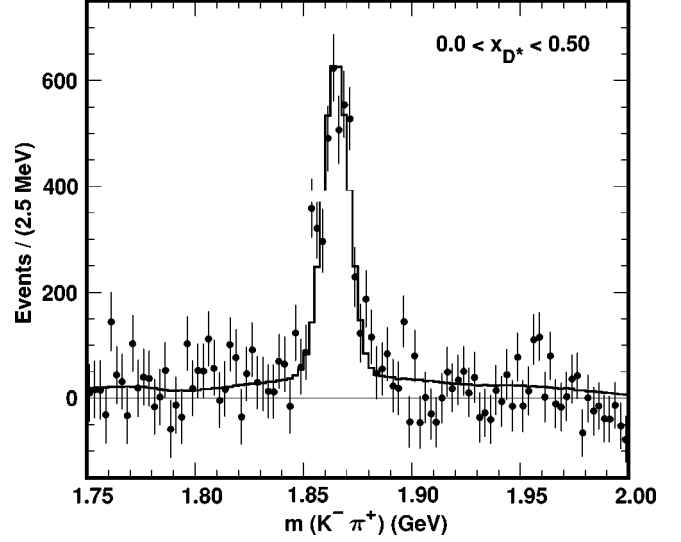
FIG. 23. The m(K^- \pi^+) distribution for D^0 candidates from B \rightarrow D^{*0}X in the momentum interval ( 0.0 < x_{D^*} < 0.50 ).
