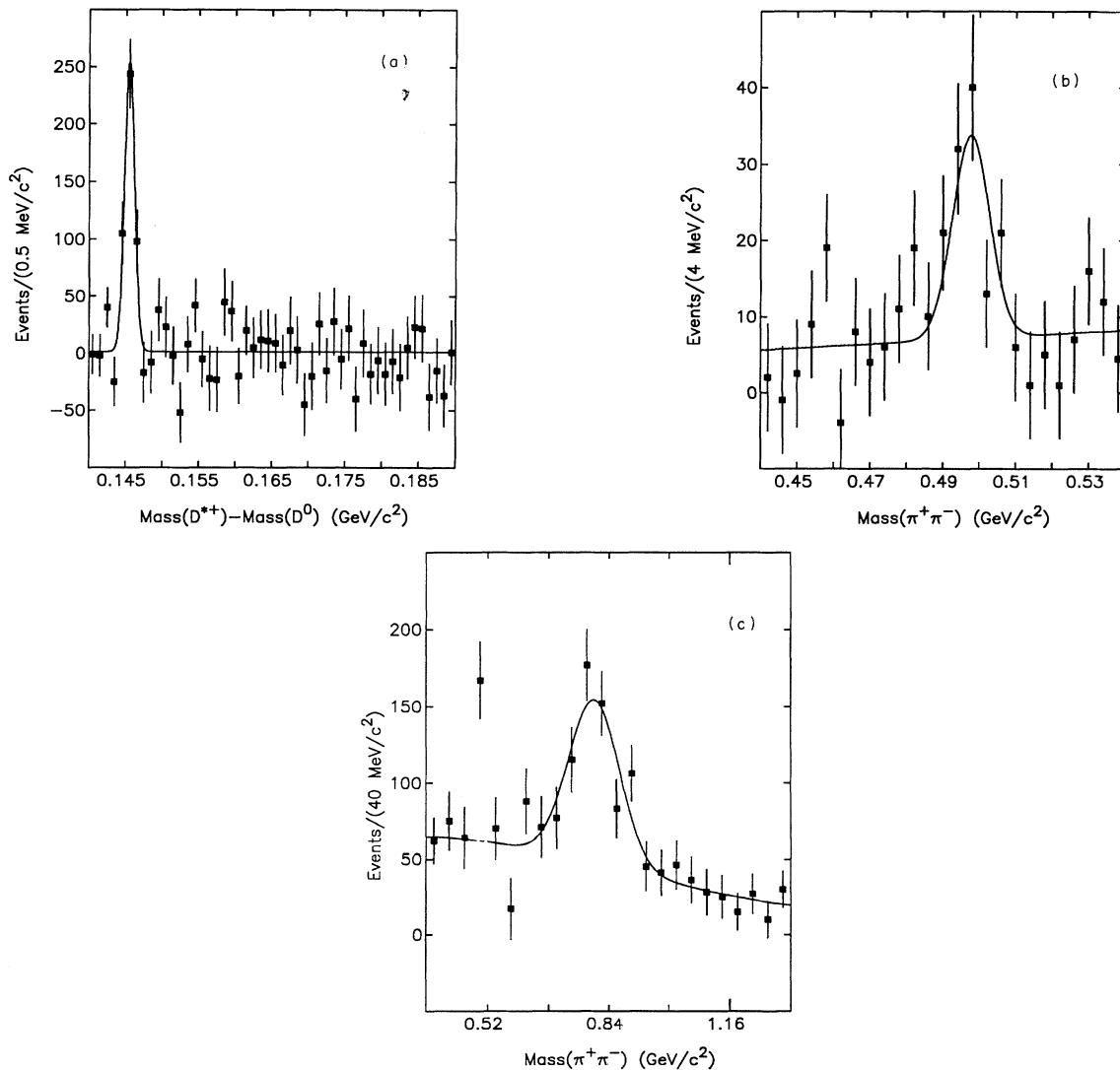
FIG. 2. (a) Background-subtracted D^{*+} - D^0 mass-difference plot, where D^0 \rightarrow \pi^+ \pi^- \pi^+ \pi^- . (b) Background-subtracted \pi^+ \pi^- mass spectrum for tracks included in the D^{*+} peak in (a); the K_S^0 region is shown. (c) Background-subtracted \pi^+ \pi^- mass spectrum for tracks included in the D^{*+} peak in (a); the \rho^0 region is shown. The fit excludes the K_S^0 region.
